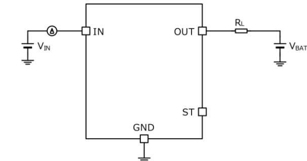
Measurement Circuit for Figure 3, Figure 4
