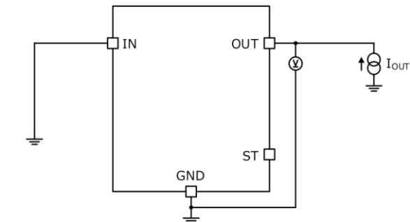
Measurement Circuit for Figure 8, Figure 9
