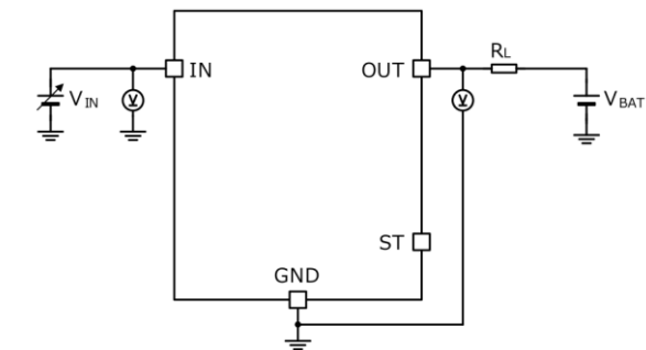
Measurement Circuit for Figure 2
