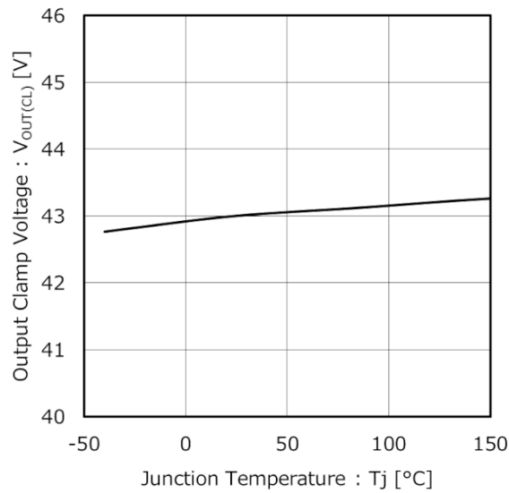
Figure 9. Output Clamp Voltage vs Junction Temperature (IOUT = 1 mA)
