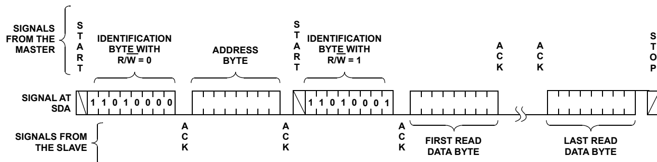
FIGURE 14. READ SEQUENCE
