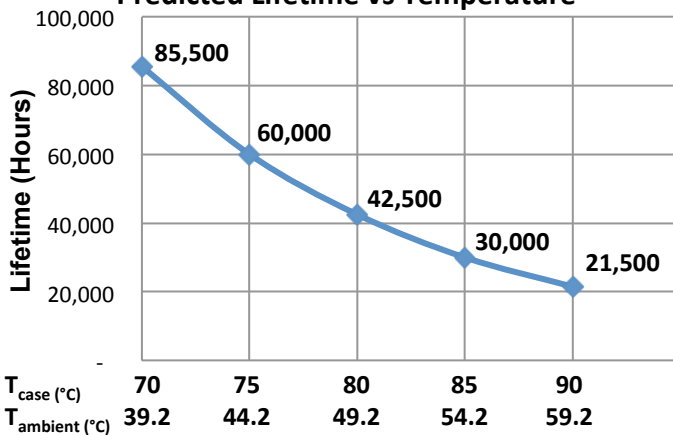
ESM050W-1200-42 (50.4 W, 1200 mA @ 42 V max) Predicted Lifetime vs Temperature
