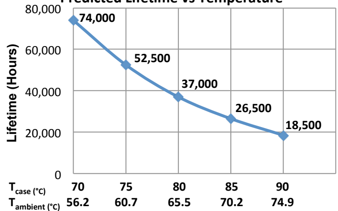
ESM040W-0700-56 (39.2 W, 700 mA @ 56 V max) Predicted Lifetime vs Temperature
