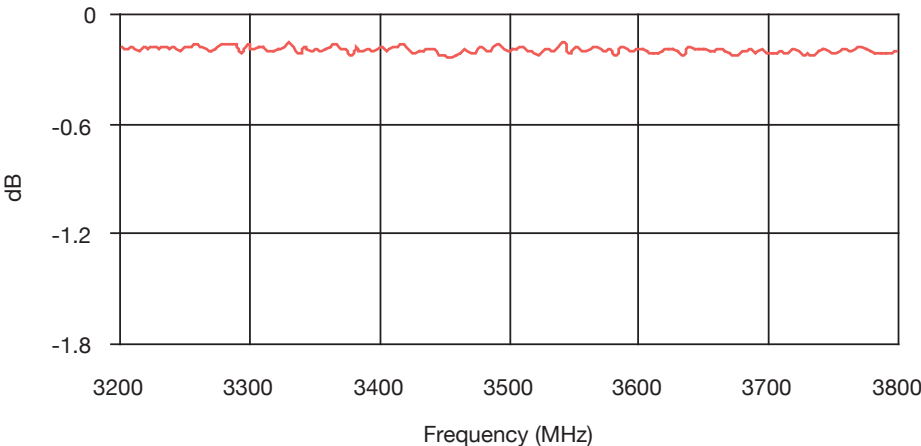
Insertion Loss
