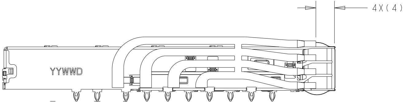
1-2331930-2 UNMARKED DIMENSIONS SAME AS 2331930-1 SCALE 3:2
