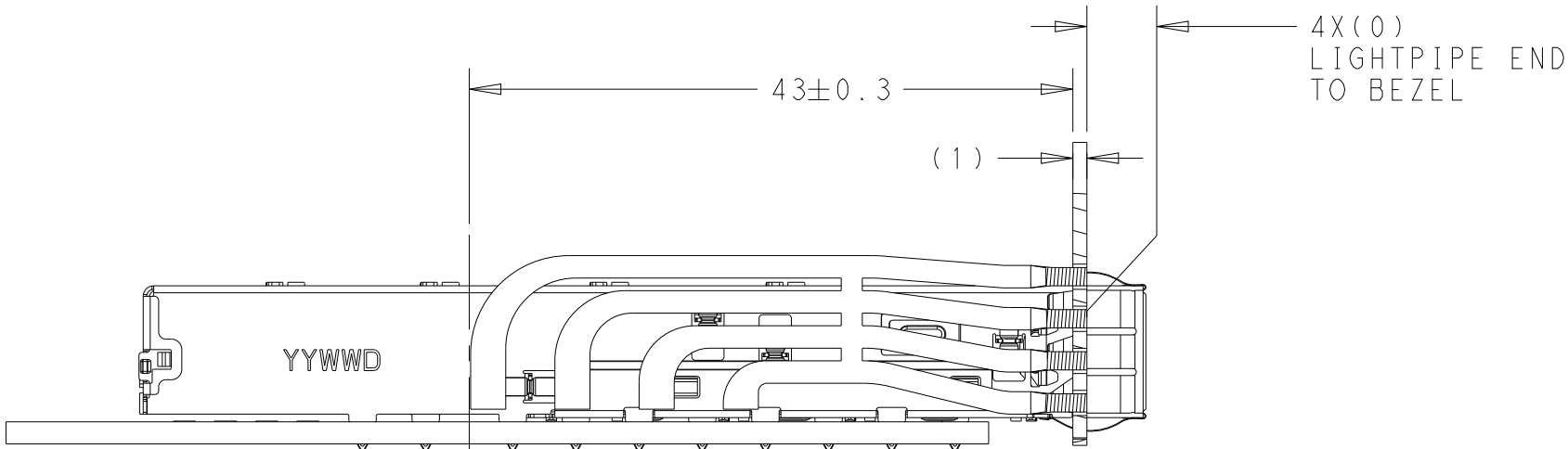
1-2331930-2 SINGLE SIDE MOUNTING
