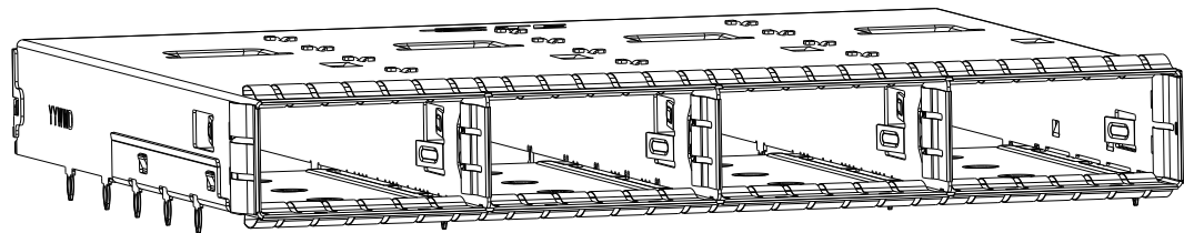
1-2331930-0 UNMARKED DIMENSIONS SAME AS 2331930-1 SCALE 3:2
