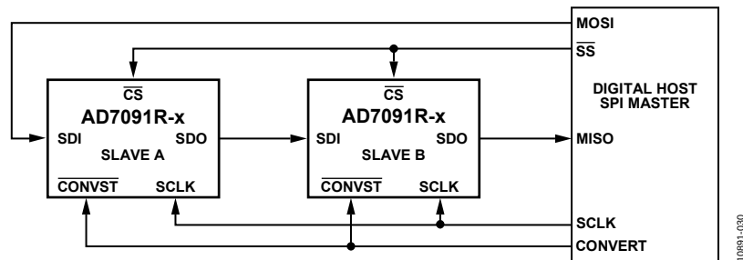
Figure 57. Daisy-Chain Configuration
