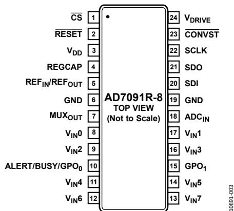
Figure 9. 8-Channel, 24-Lead TSSOP Pin Configuration
