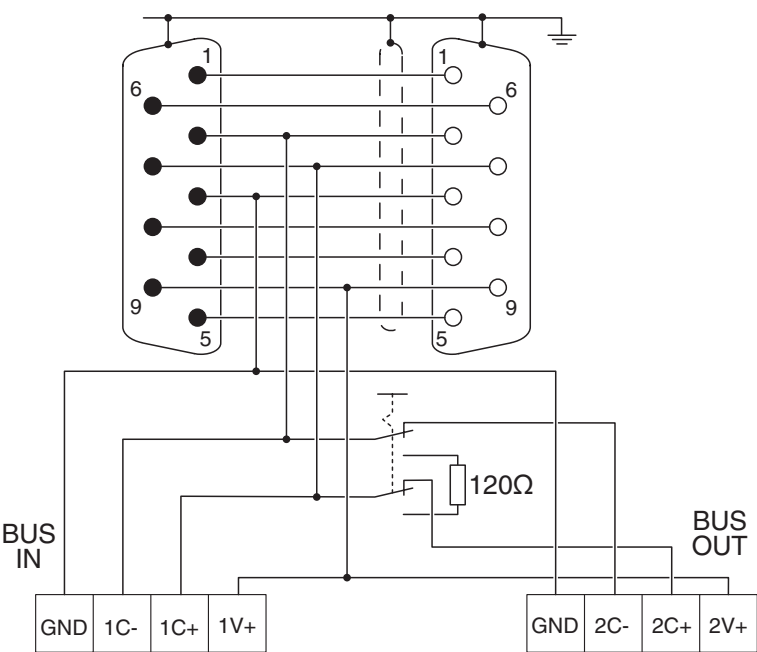
Circuit diagram
