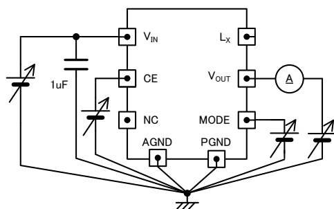
< Circuit ⑦ >
