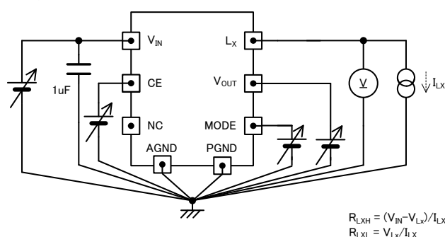
< Circuit ④ >
