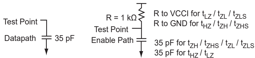
FIGURE 2-10: AC LOADING
