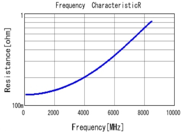
■ GCQ1555C1H3R5WB01 R DC0V, 25degC
