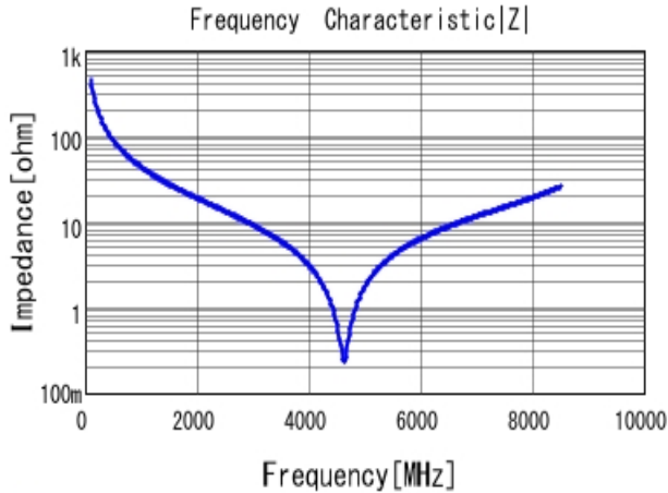
■ GCQ1555C1H3R5WB01 |Z| DC0V, 25degC
