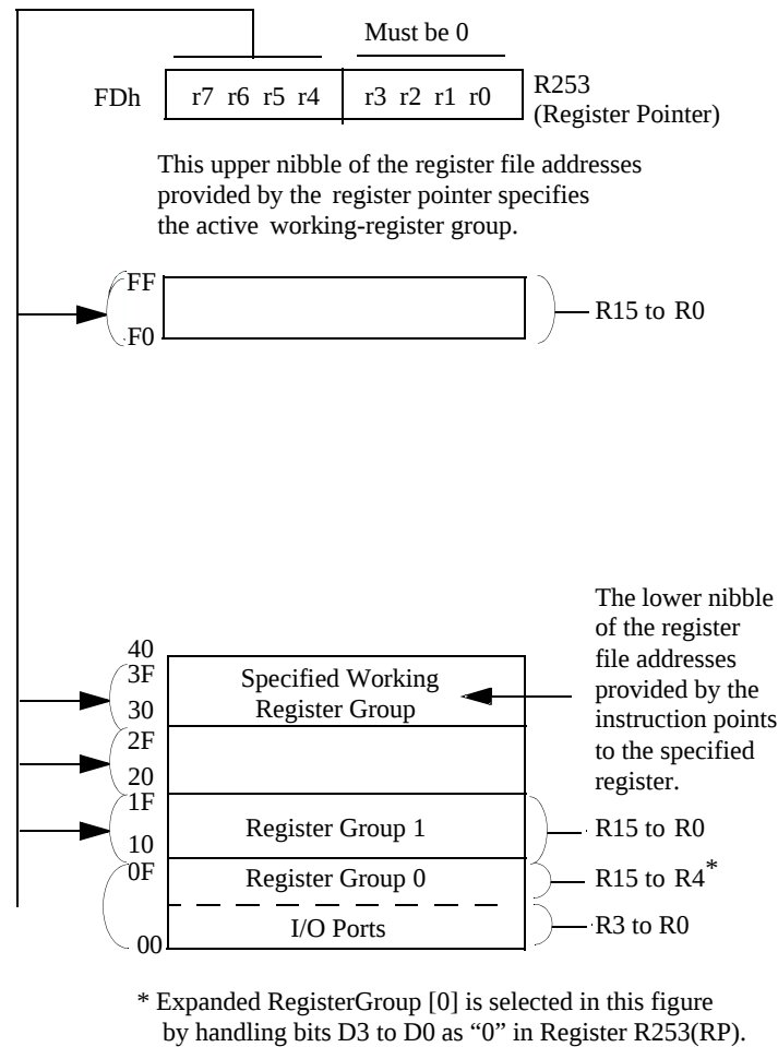
Figure 15. Register Pointer
