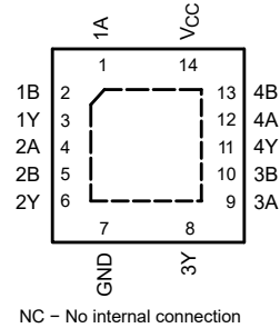
Figure 5-2. SN74AHC86 RGY Package, VQFN 14-Pin (Top View)
