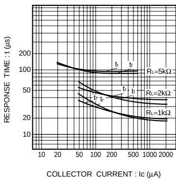
Fig.8 Response time vs. collector current
