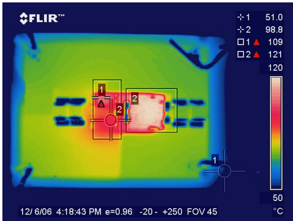
Image 7 – Vin: 12V Iout: 8Amps Ambient Temp: 25°C Airflow: 0lfm Pdiss: 3.73W
