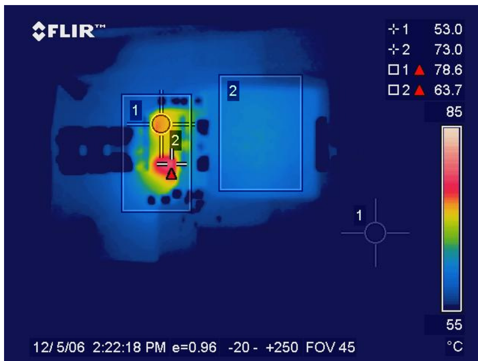
Image 6 – Vin: 12V Iout: 10Amps Ambient Temp: 25°C Airflow: 100lfm Pdiss: 2.84W
