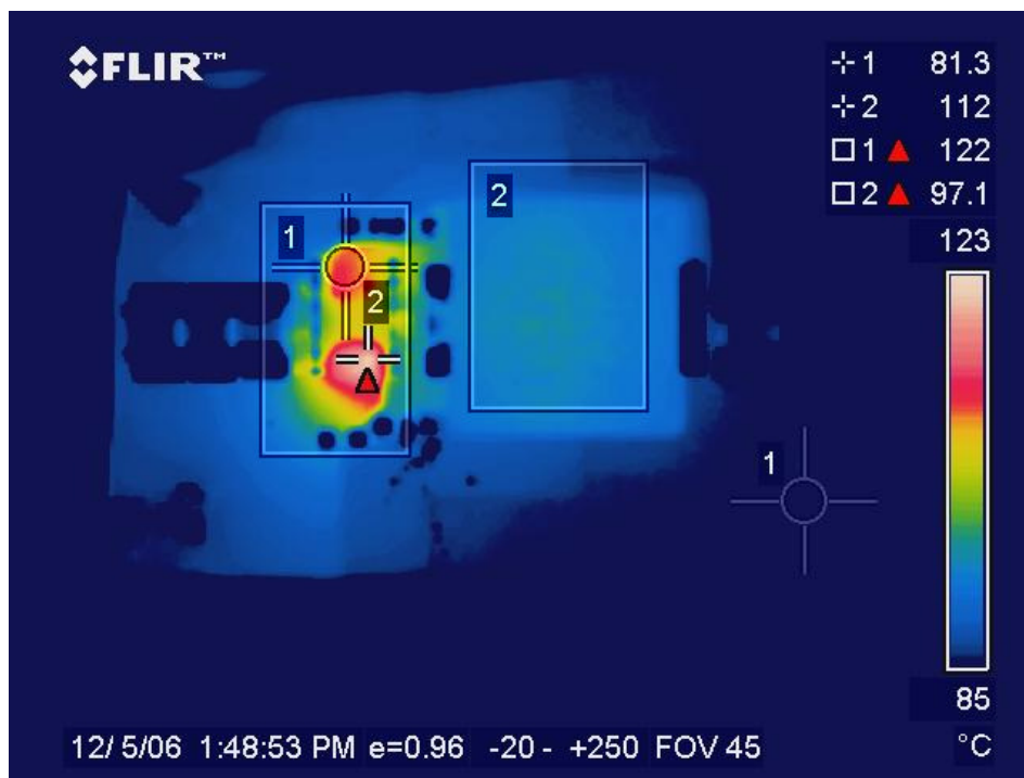
Image 5 – Vin: 12V Iout: 12Amps Ambient Temp: 25°C Airflow: 0lfm Pdiss: 3.65W
