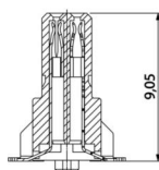
12 Pins
