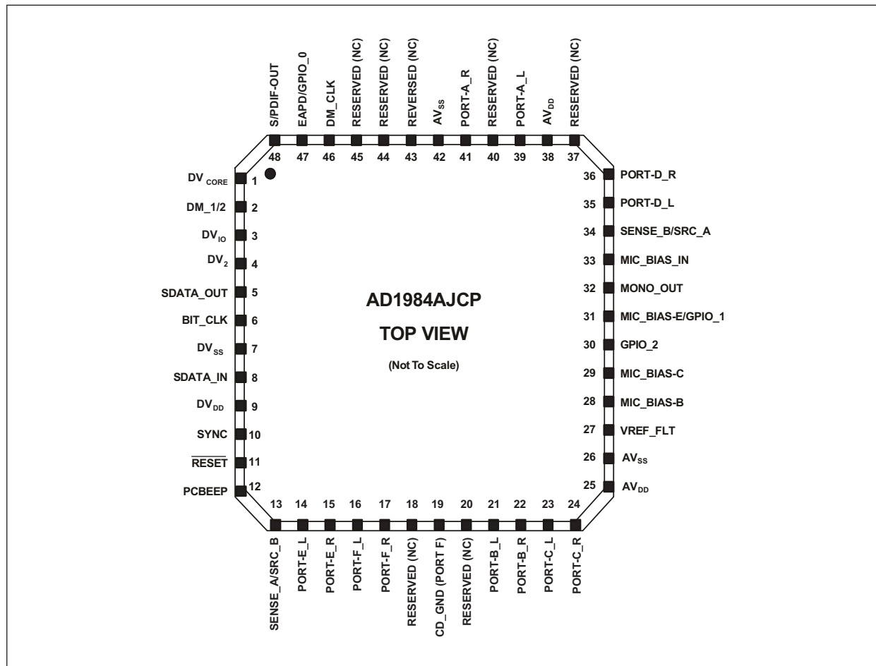
Figure 1. AD1984A Pinout
