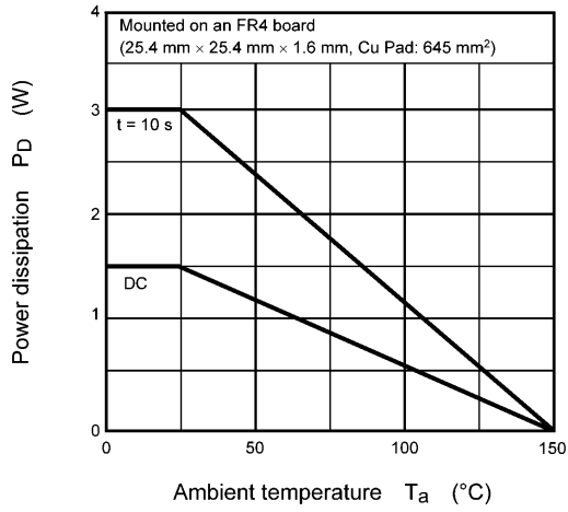
Fig. 8.13 P_D - T_a
