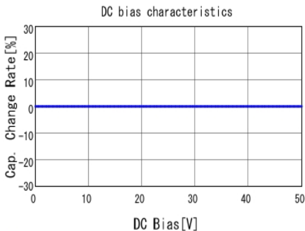
■ GCQ1555C1H8R2DB01 C-DC bias capchange, 25.0degC, AC1V
