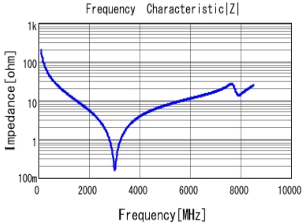
■ GCQ1555C1H8R2DB01 |Z| DC0V, 25degC
