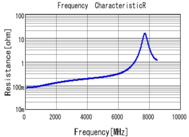
■ GCQ1555C1H8R2DB01 R DC0V, 25degC
