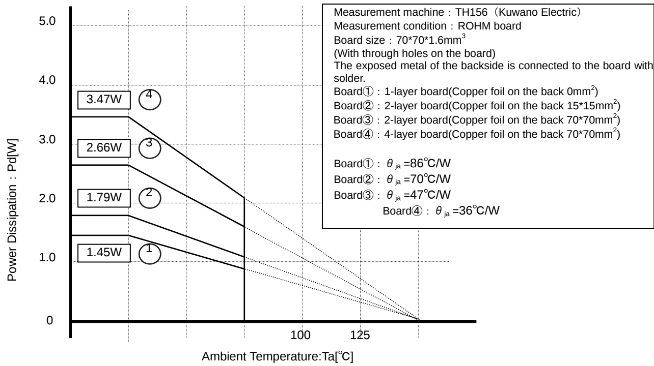
Fig. 2 HSOP25 Derating curve
