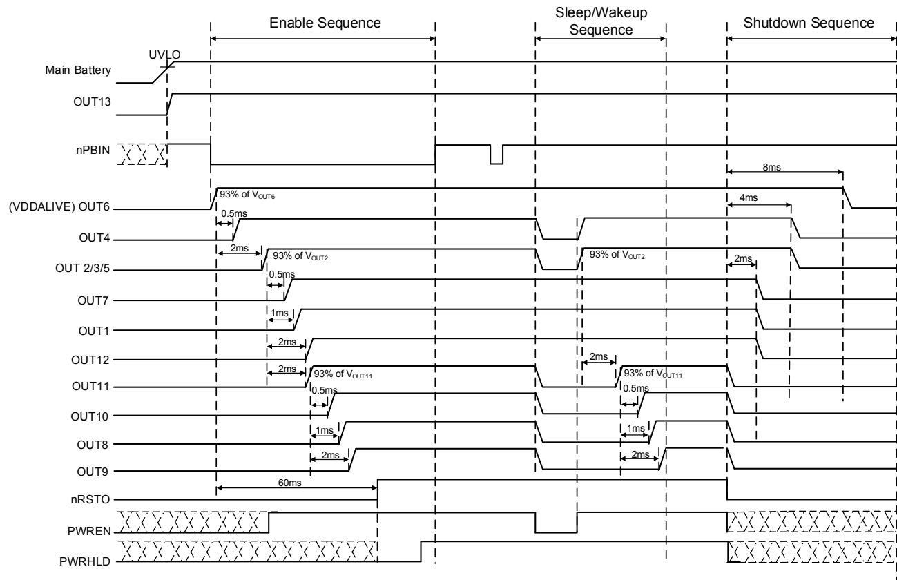
Figure 3: Power Control Sequence
