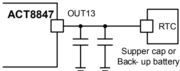
Figure 5: Typical Application of RTC LDO
