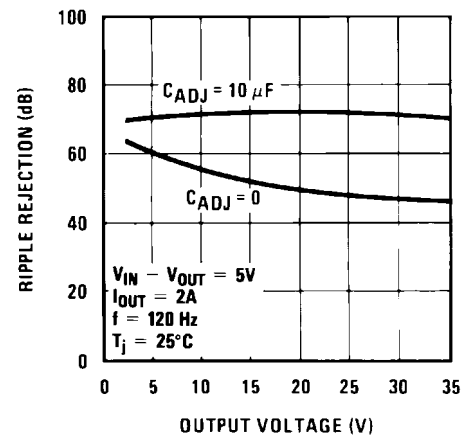
Figure 10. Ripple Rejection
