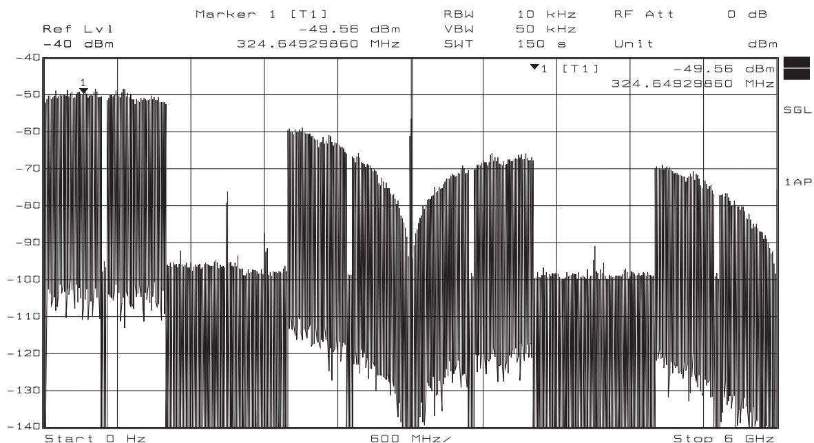
Figure 7-51. Spectrum over 4 Nyquist Zones at 3 Gps in NRZ Output Mode
