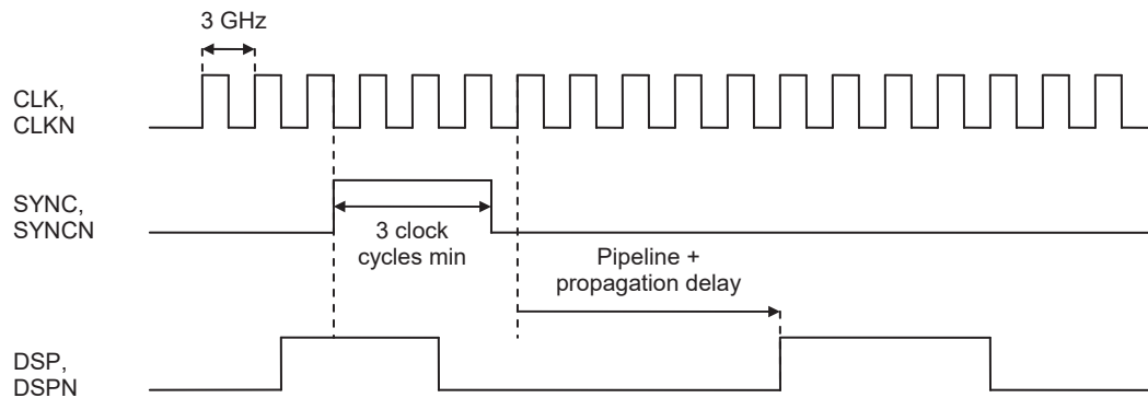
Figure 5-14. Reset Timing Diagram (4:1 MUX)
