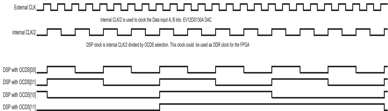
Figure 5-11. OCDS Timing Diagram for 2:1 MUX
