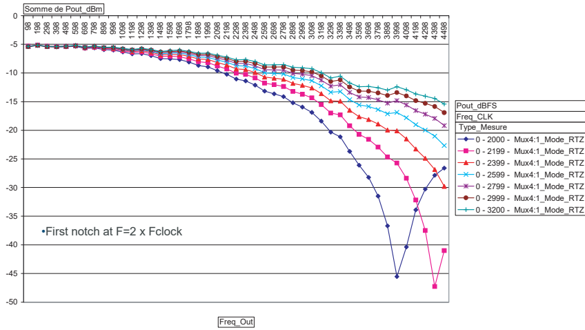
Figure 7-8. Available Pout vs Fout from 98 MHz to 4498 MHz and from 2 Gbps to 3.2 Gbps in RTZ Mode
