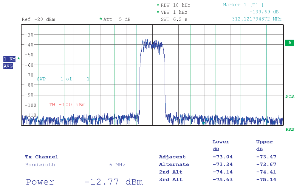
Figure 7-37. ACPR 1 channel centered on 300 MHz, Output Mode NRTZ
