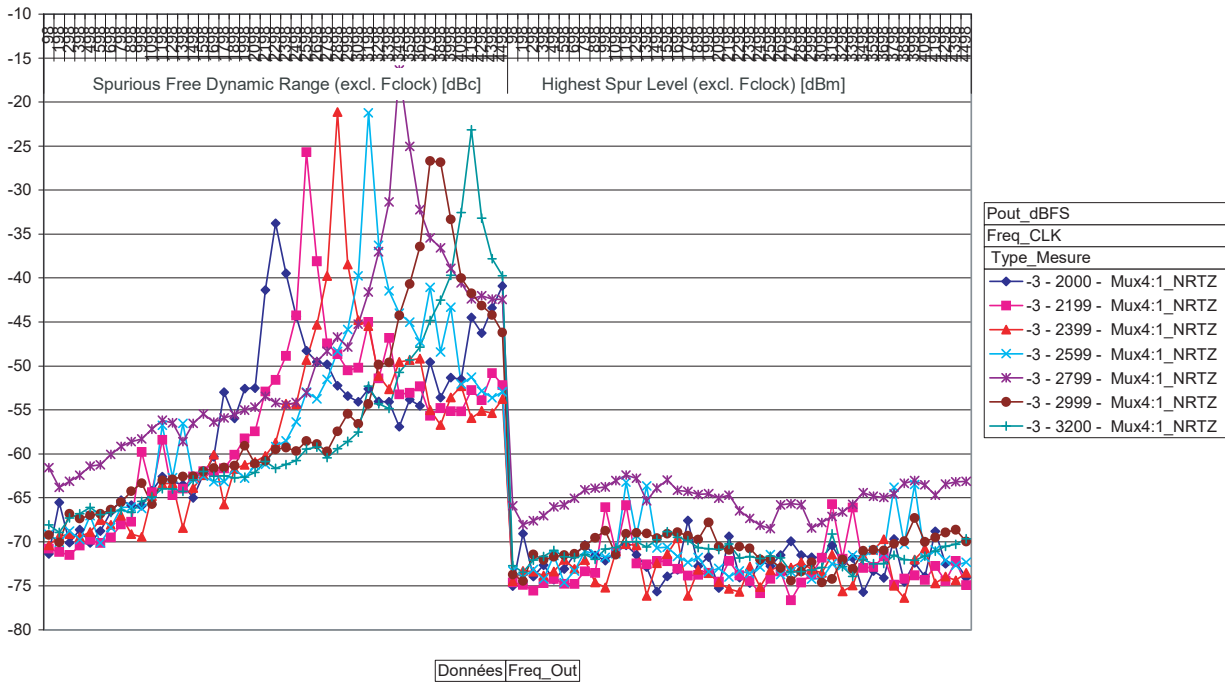
Figure 7-11. SFDR and HSL in NRTZ mode at -3 dBFS for Sampling Rate from 2000 MSps to 3200 MSps
