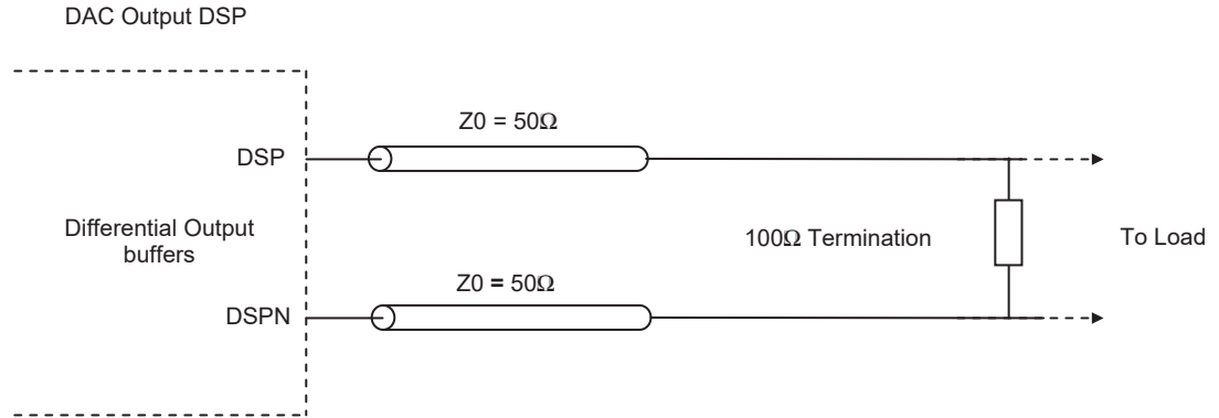
Figure 8-6. DSP Output Differential Termination
