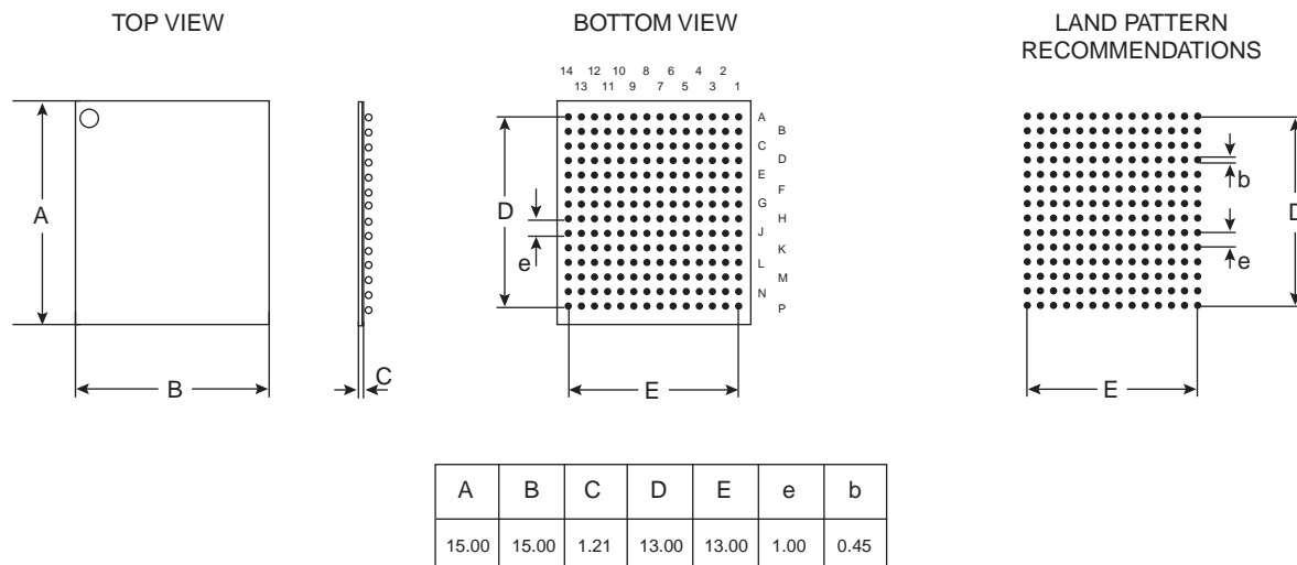
Figure 9-1. Land Pattern Recommendation
