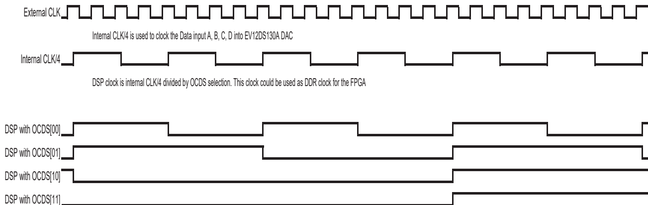
Figure 5-10. OCDS Timing Diagram for 4:1 MUX
