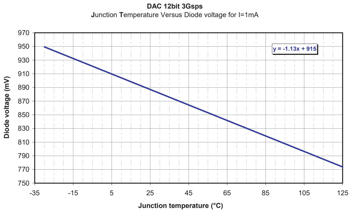
Figure 5-17. Diode Characteristics for Die Junction Monitoring
