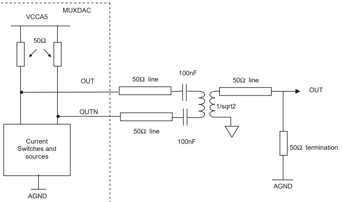
Figure 8-2. Analog Output Using a 1/\sqrt{2} Balun
