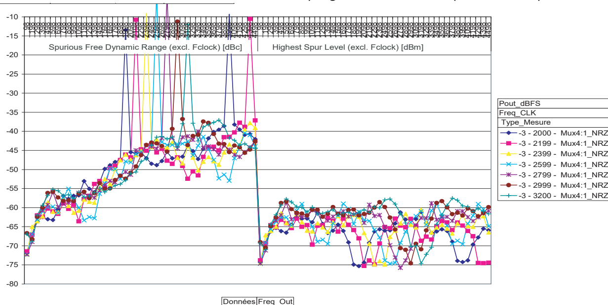
Figure 7-10. SFDR and HSL in NRZ mode at -3 dBFS for Sampling Rate from 2000 MSps to 3200 MSps
