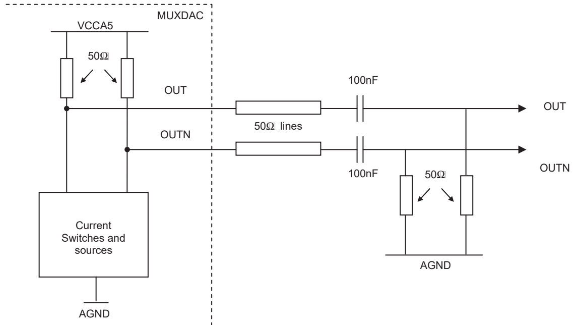
Figure 8-1. Analog Output Differential Termination
