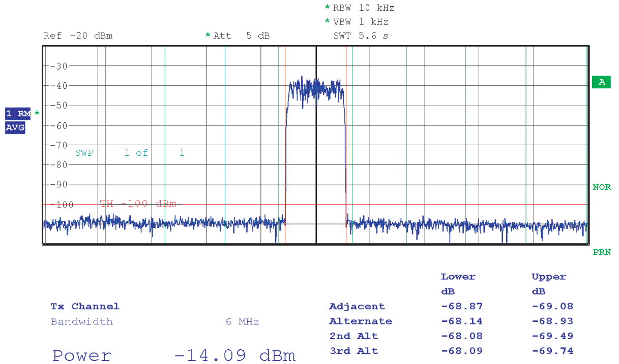
Figure 7-36. ACPR 1 Channel Centered on 900 MHz, Output Mode NRTZ
