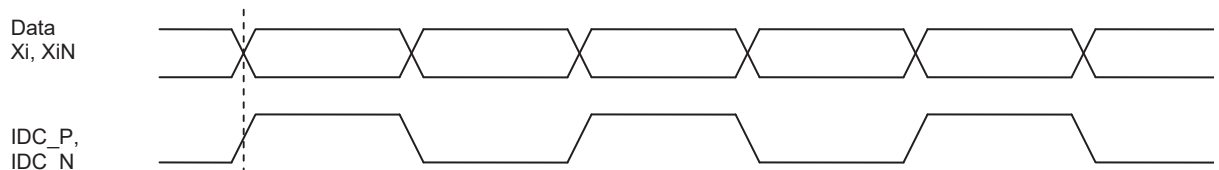
Figure 5-12. IDC Timing vs Data Input
