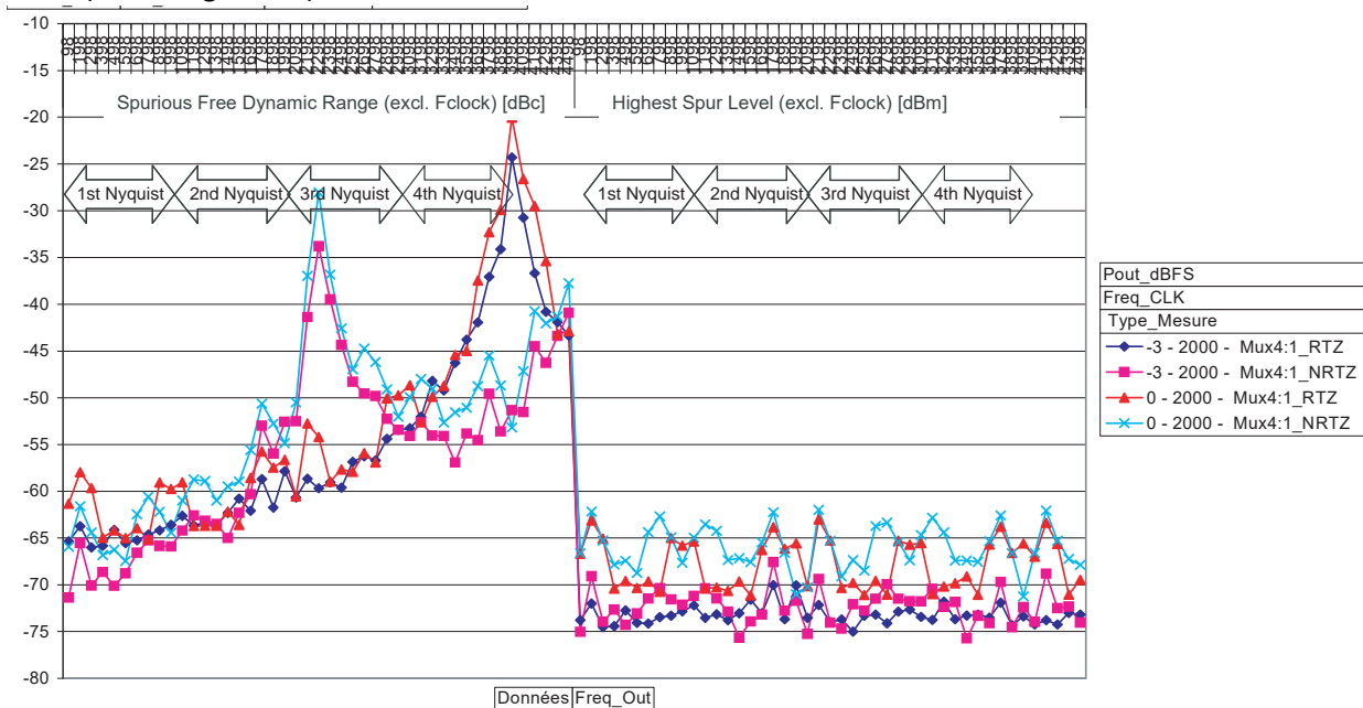
Figure 7-20. Comparison of NRTZ and RTZ Modes at Full Scale and -3 dBFS at 2000 MSps: SFDR and HSL (Excluding Fclock)
