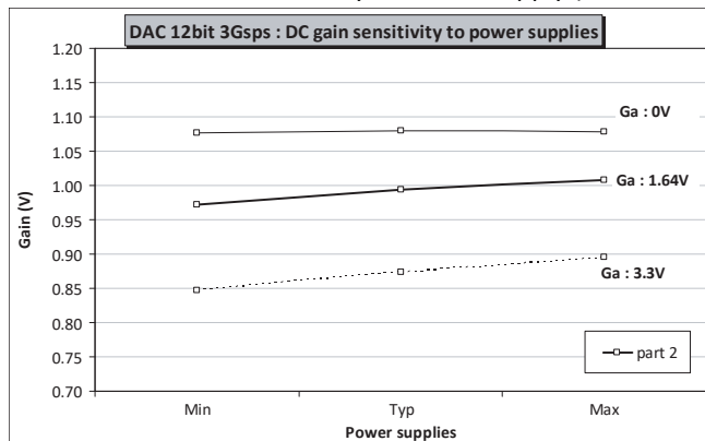
Figure 7-3. DC Gain Sensitivity to Power Supply (Measured in NRZ Output Mode)
