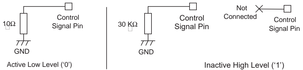
Figure 8-7. Control Signal Settings
