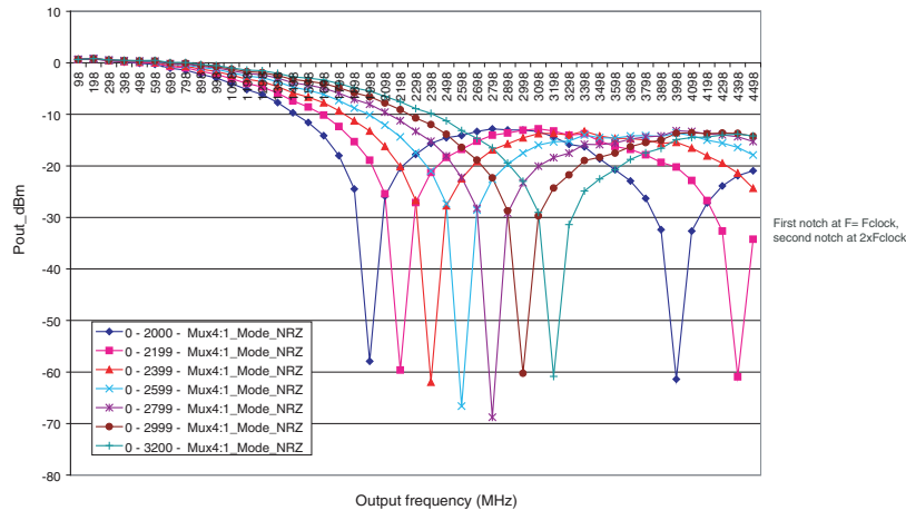
Figure 7-6. Available Pout vs Fout from 98 MHz to 4498 MHz and from 2 Gps to 3.2 Gps in NRZ Mode
