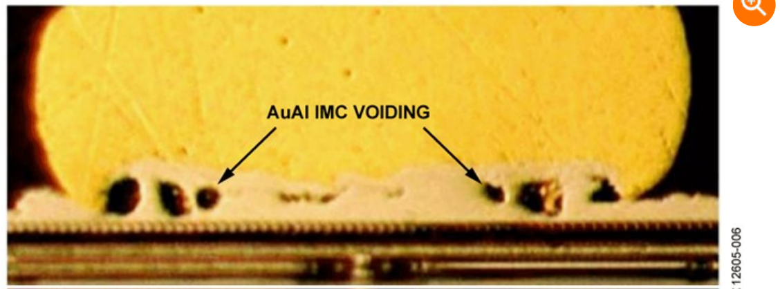
Figure 6. Au Ball Bond on Al Pad, After 500 Hours at 195°C
