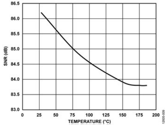
Figure 9. SNR over Temperature, 1 kHz Input Tone, 580 kSPS
