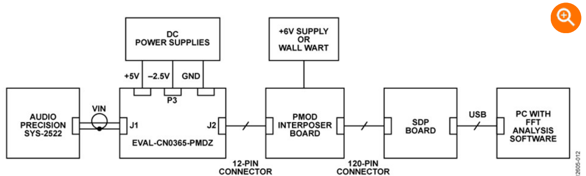
Figure 12. Circuit Test Setup for Measuring AC Performance
