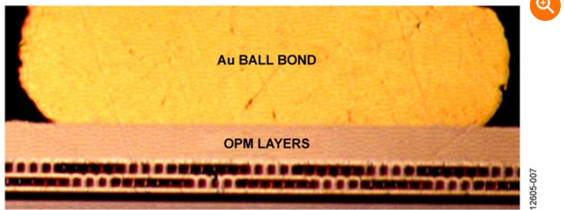
Figure 7. Au Ball Bond on OPM Pad, After 6000 Hours at 195°C
