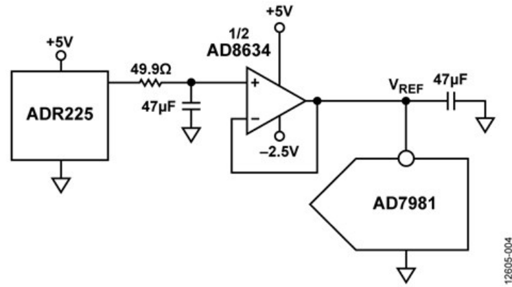
Figure 4. SAR ADC Reference Buffer and RC Filter
