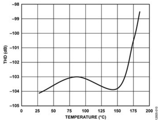
Figure 10. THD over Temperature, 1 kHz Input Tone, 580 kSPS
