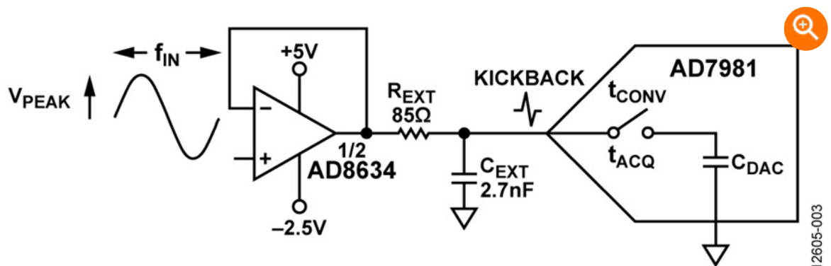
Figure 3. SAR ADC Front End Amplifier and RC Filter
