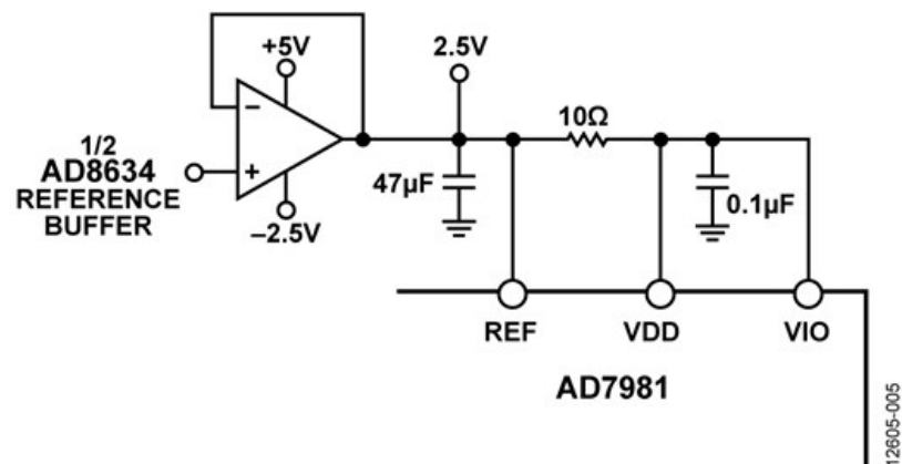
Figure 5. Supplying ADC Reference from Reference Buffer
