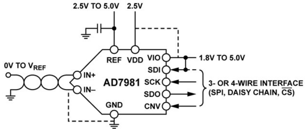
Figure 2. AD7981 Connection Diagram
