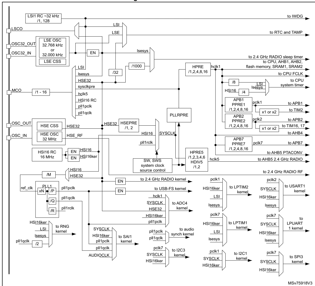
Figure 6. Clock tree
