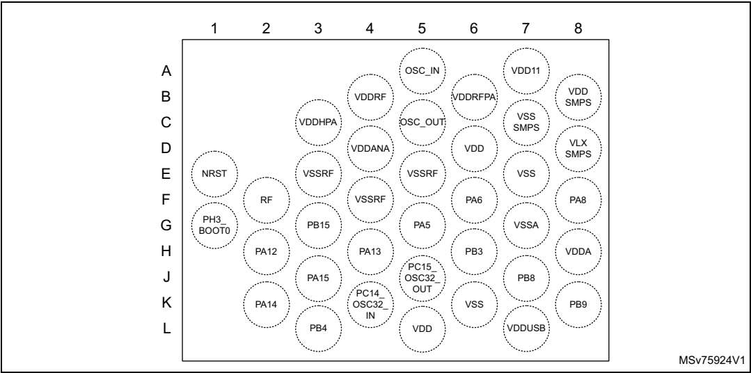
Figure 10. Thin WLCSP37 SMPS USB ballout (1)
