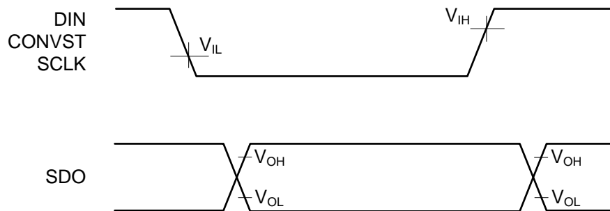
Figure 44. Voltage Levels for Timing
