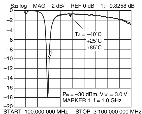
S 22 -FREQUENCY
