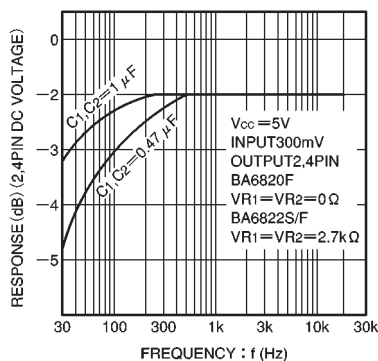
Fig. 10 Frequency characteristics
