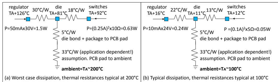
Figure 15. Example of thermal power dissipation estimation
