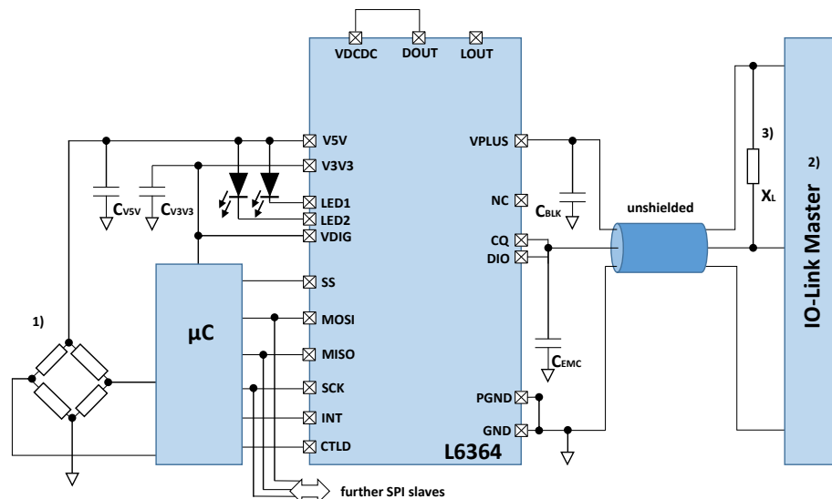
Figure 21. Typical IO-Link Sensor application, DCDC bypassed, CQ and DIO in JOIN mode (coupled), VDIG = V3V3
