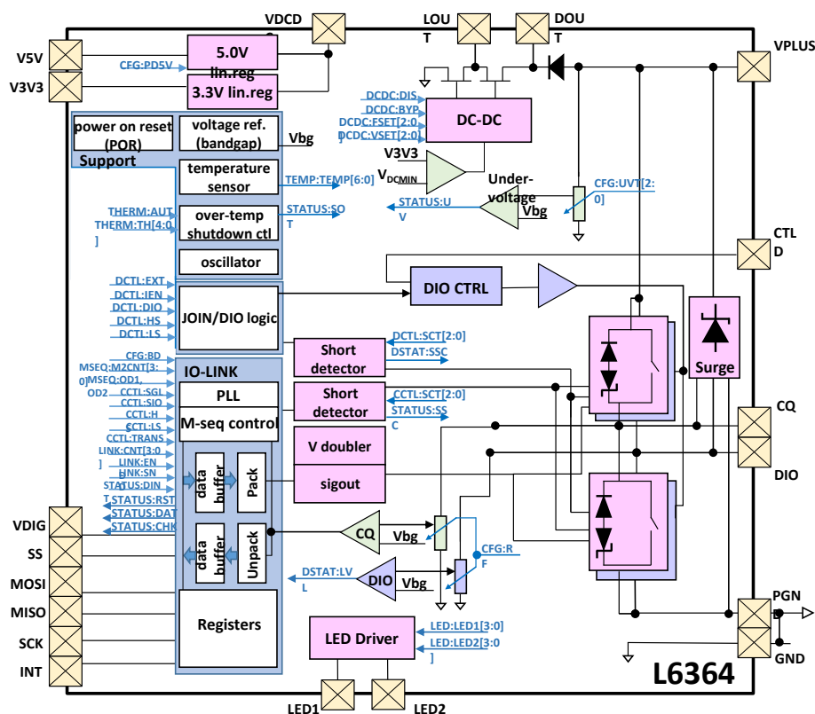
Figure 19. Detailed block diagram, showing register field connections
