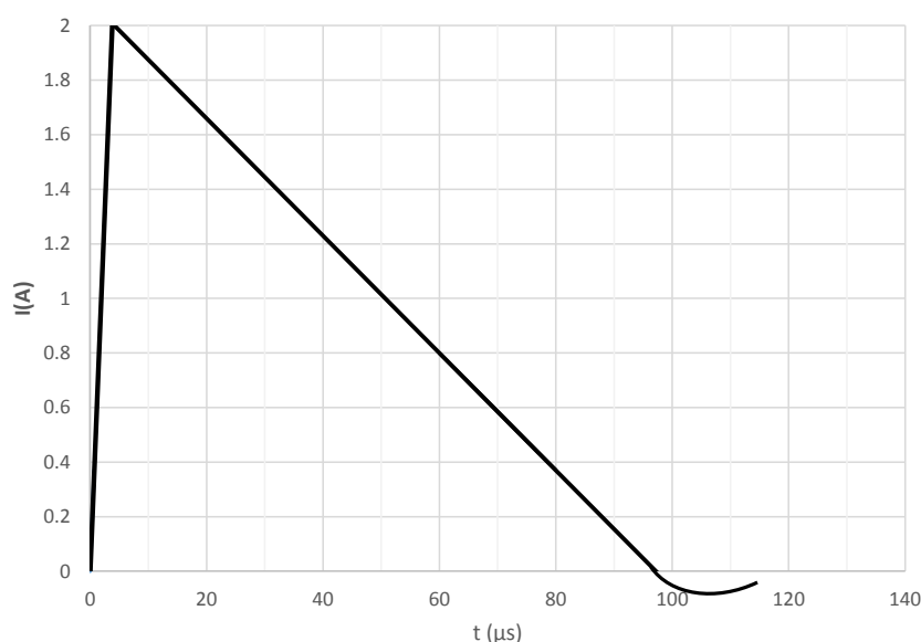
Figure 16. Surge waveform
