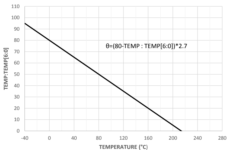
Figure 8. L6364 temperature measurement
