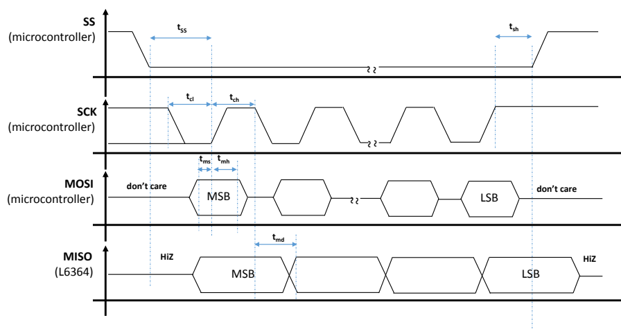
Figure 3. Register programming.
