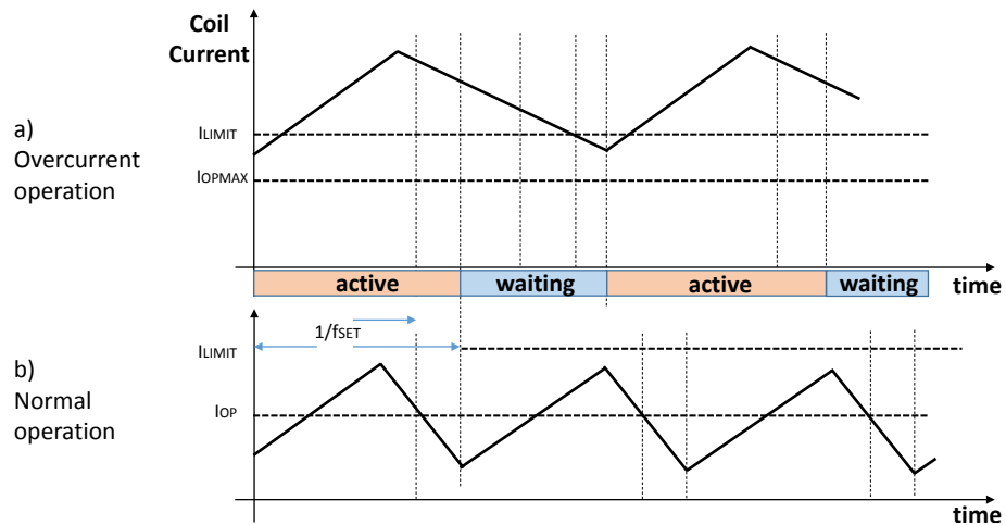
Figure 13. Overcurrent operation
