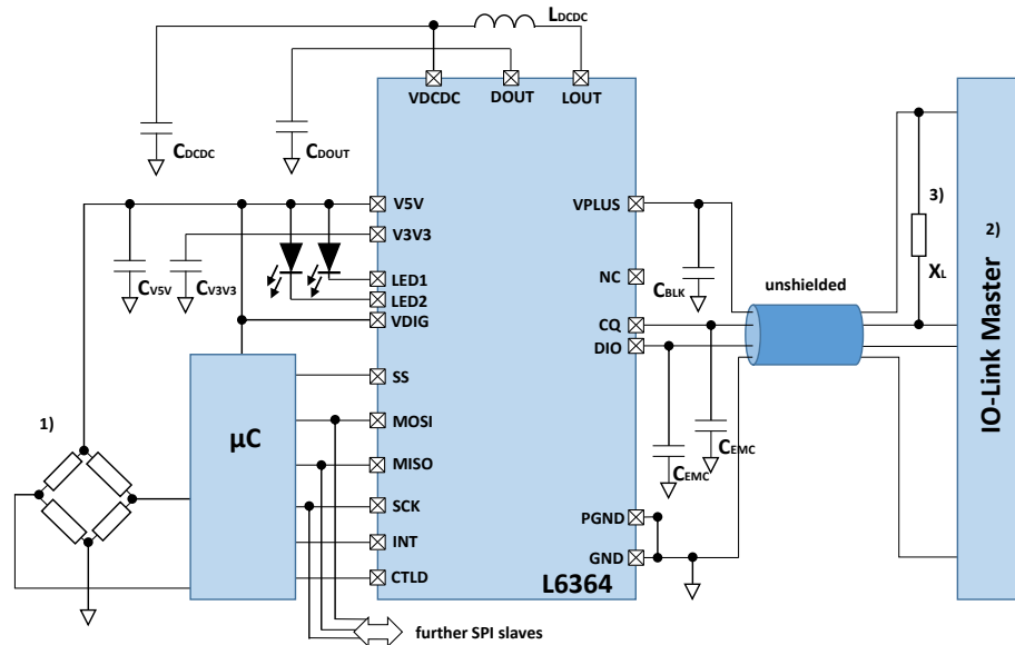
Figure 20. Typical IO-Link Sensor application, DCDC in use, CQ and DIO outputs in DIO mode (independent), VDIG = V5V
