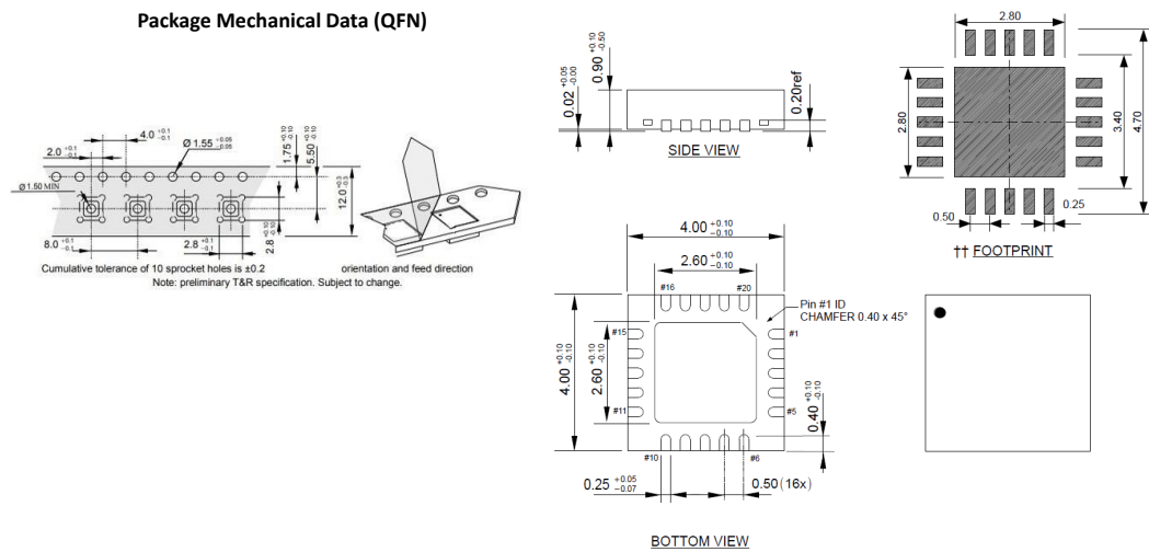
Figure 22. Package, footprint and tape drawings for QFN
