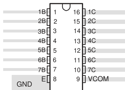
Figure 8-8. Package Layout
