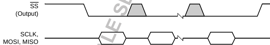
Figure 19-30. SPI 1 Master “Don’t Care” DATA_READY Timing Diagram
