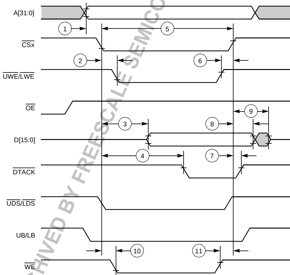
Figure 19-3. Chip-Select Write Cycle Timing Diagram
