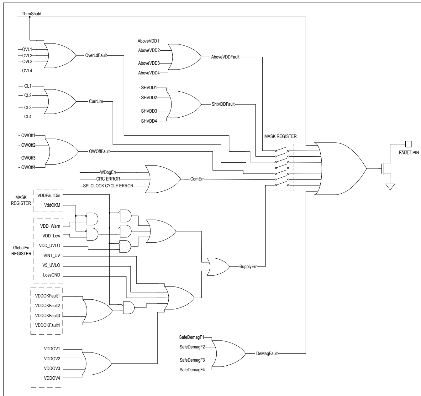
Figure 6. FAULT Interrupt Sources
