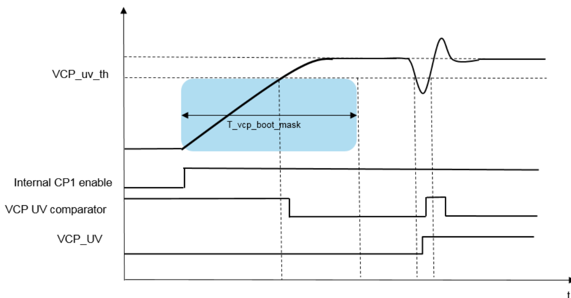
Figure 31. VCP UV boot masking
