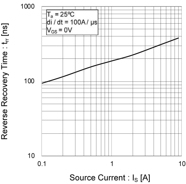
Fig.19 Reverse Recovery Time vs. Source Current
