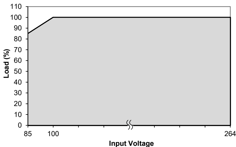
Fig. 2 De-rating for AC Input Voltage < 100 Vac de-rate power by 1 % / Vac
