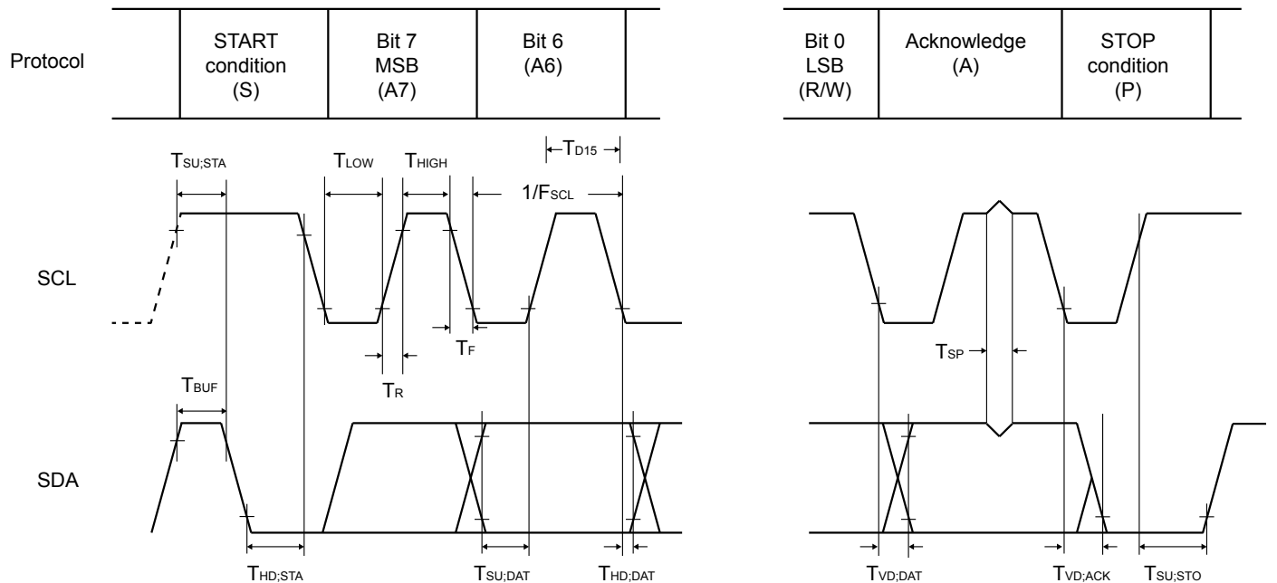
Figure 2. I 2 C-Bus Timing Diagram
