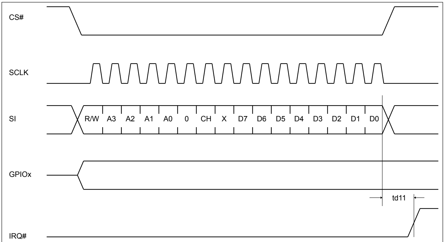
Figure 12. SPI Write THR To Clear TX INT
