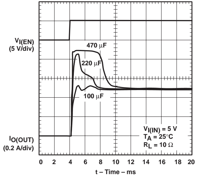
Figure 9. Inrush Current with 100-μF, 220-μF and 470-μF Load Capacitance
