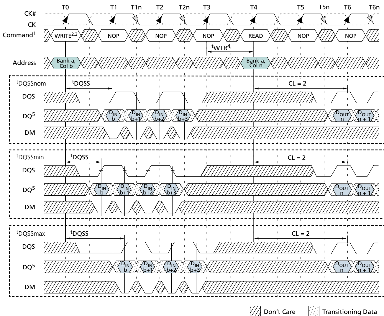
Figure 44: WRITE-to-READ – Uninterrupting
