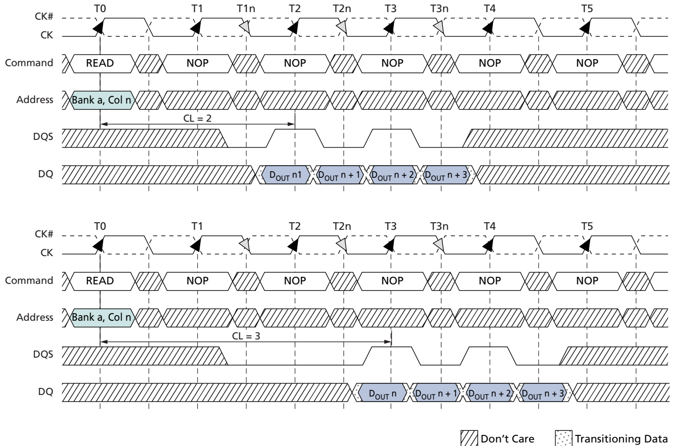
Figure 28: READ Burst
