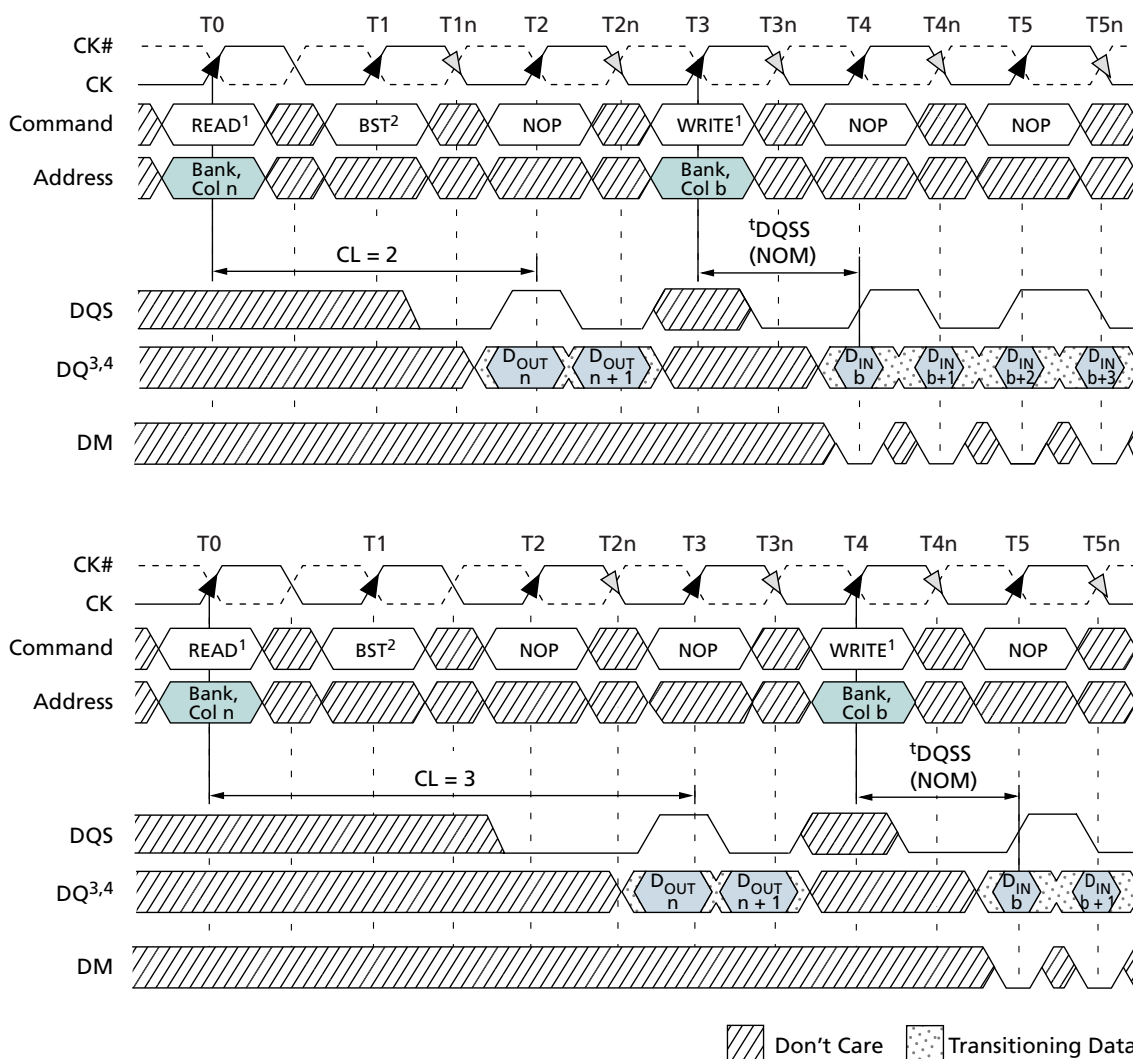
Figure 33: READ-to-WRITE
