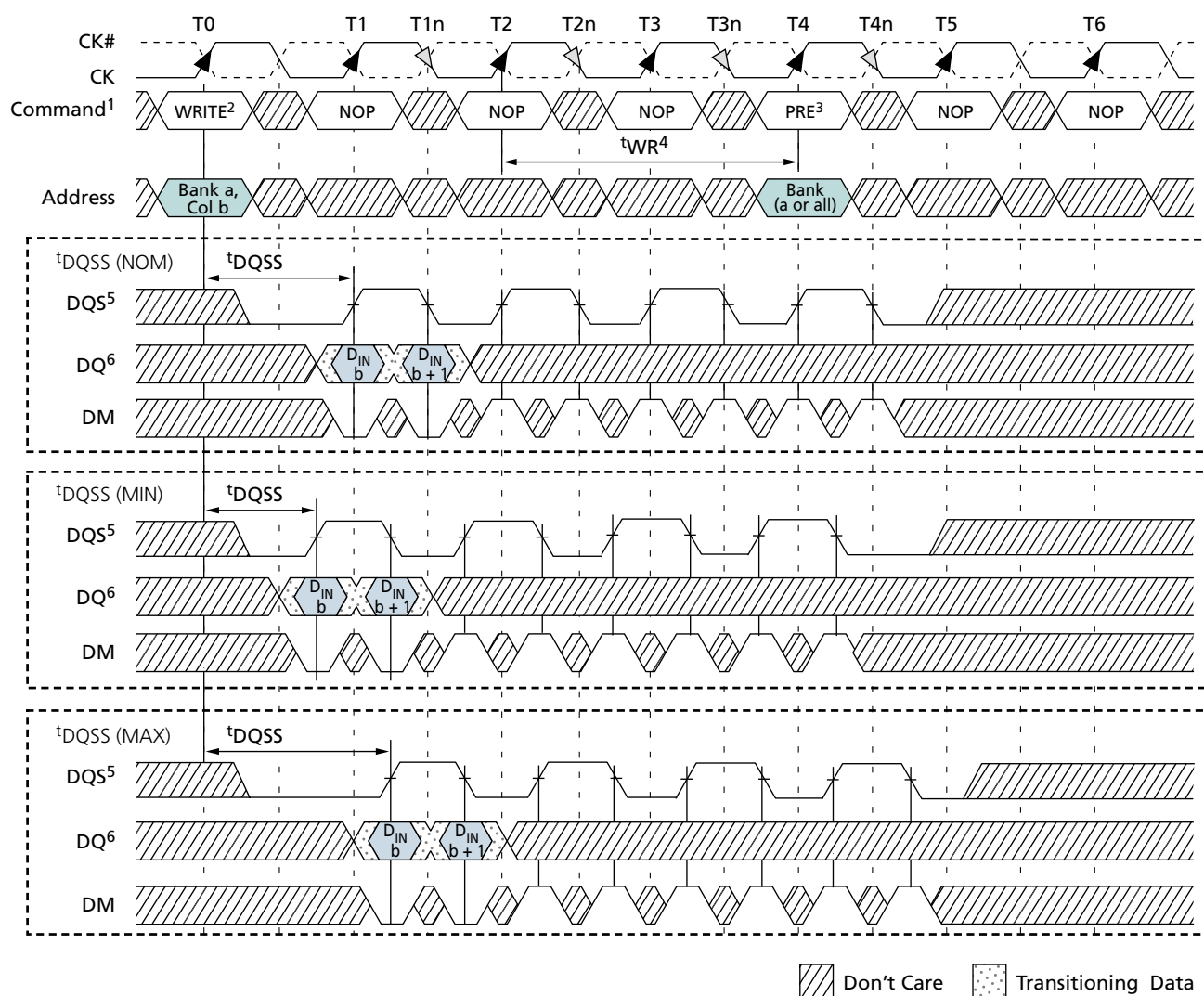
Figure 48: WRITE-to-PRECHARGE – Interrupting
