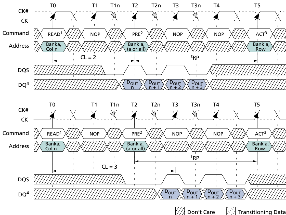
Figure 34: READ-to-PRECHARGE
