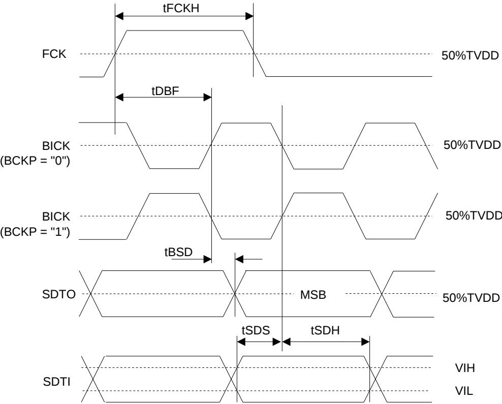
Figure 4. Audio Interface Timing (PLL/EXT Master mode, DSP mode, MSBS bit= "0")
