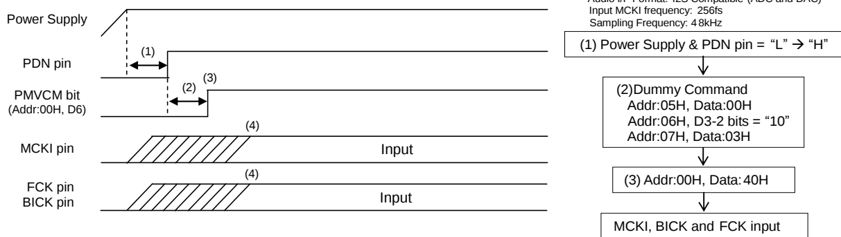
Figure 68. Clock Set Up Sequence (3)
