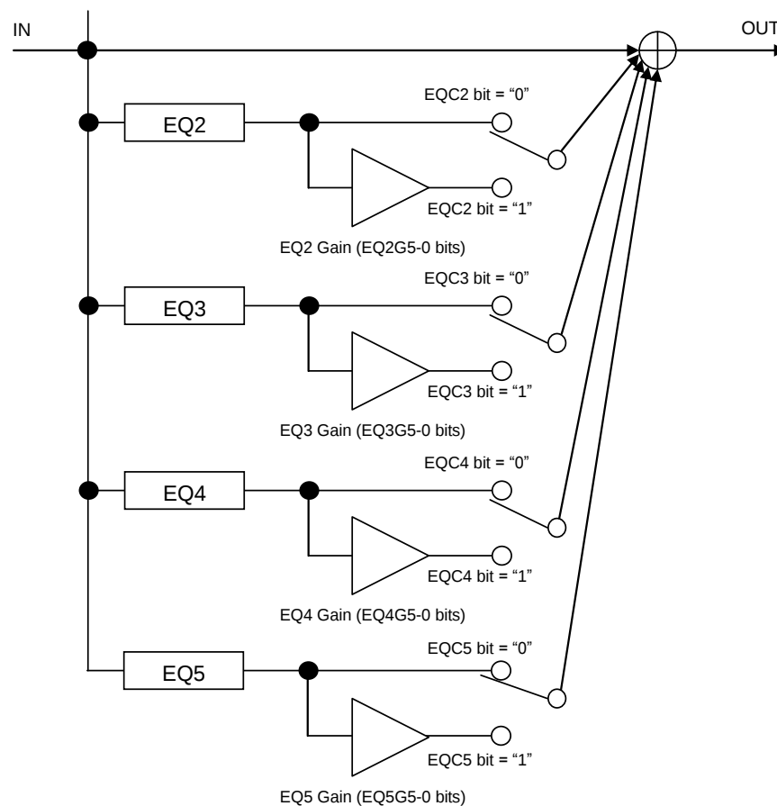
Figure 44. 4-Band EQ Structure
