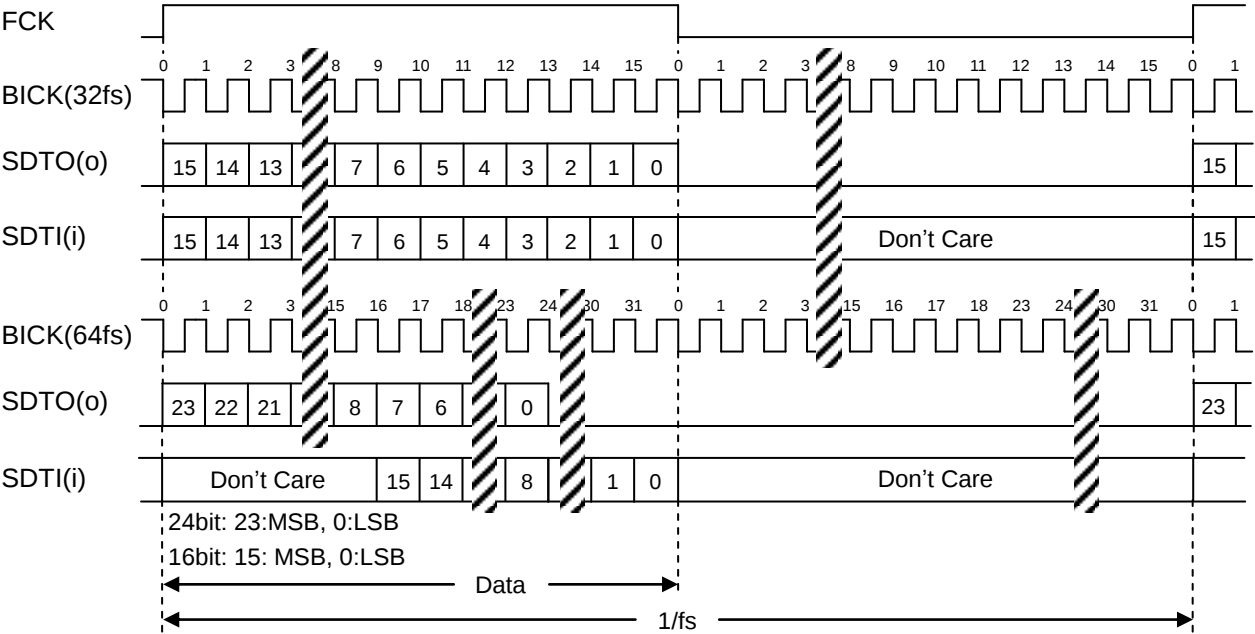
Figure 31. Mode 1 Timing
