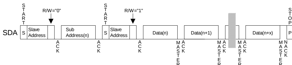
Figure 61. Random Address Read
