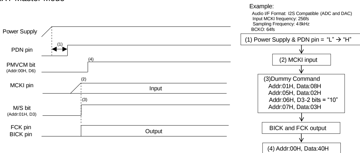
Figure 69. Clock Set Up Sequence (4)
