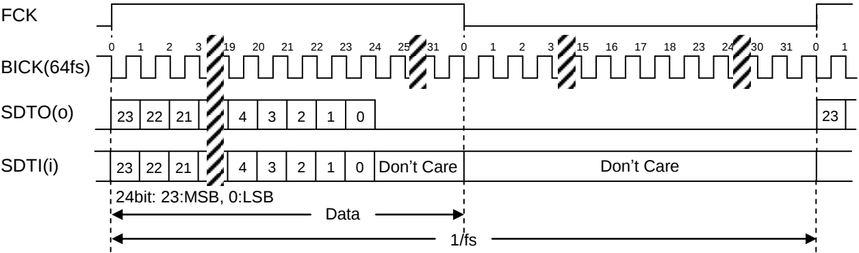
Figure 32. Mode 2 Timing
