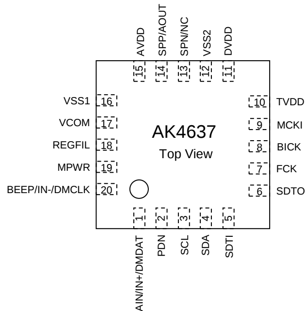
Figure 2. Pin Layout
