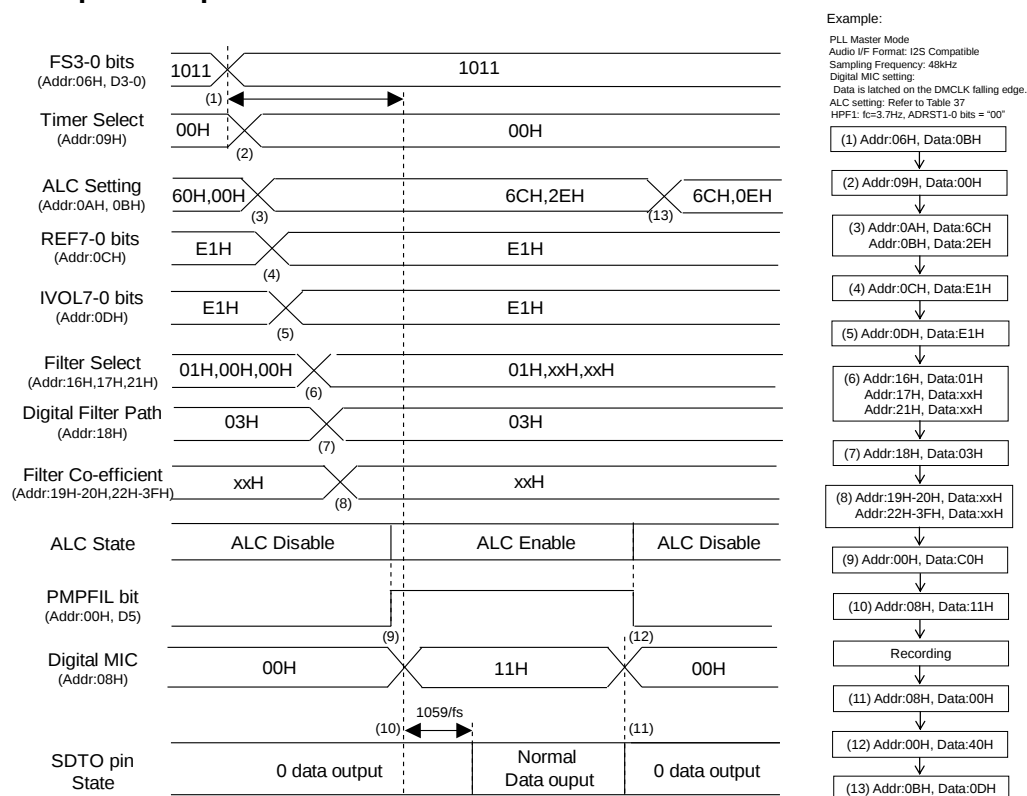
Figure 71. Digital Microphone Input Recording Sequence
