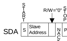
Figure 26. Reset Completion for example
