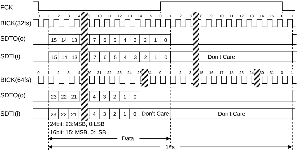
Figure 33. Mode 3 Timing
