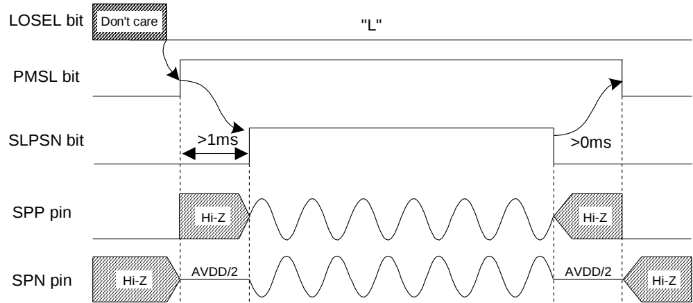
Figure 50. Power-up/Power-down Timing for Speaker-Amp
