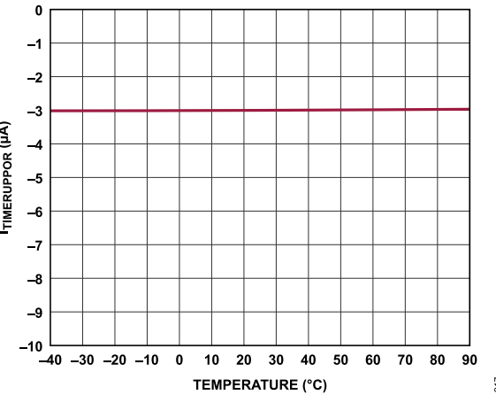
Figure 17. TIMER Pull-Up Current POR ( I_{TIMERUPPOR} ) vs. Temperature
