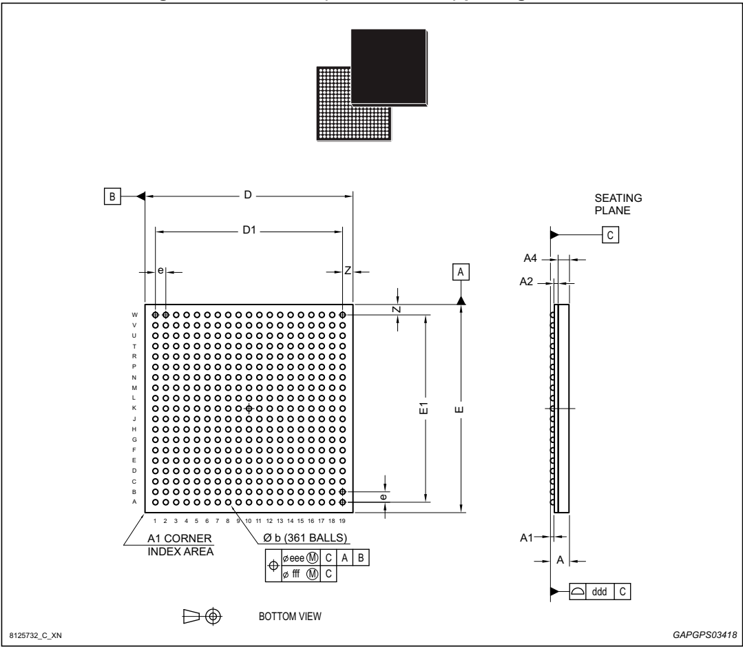
Figure 5. LFBGA361 (16x16x1.7 mm) package outline
