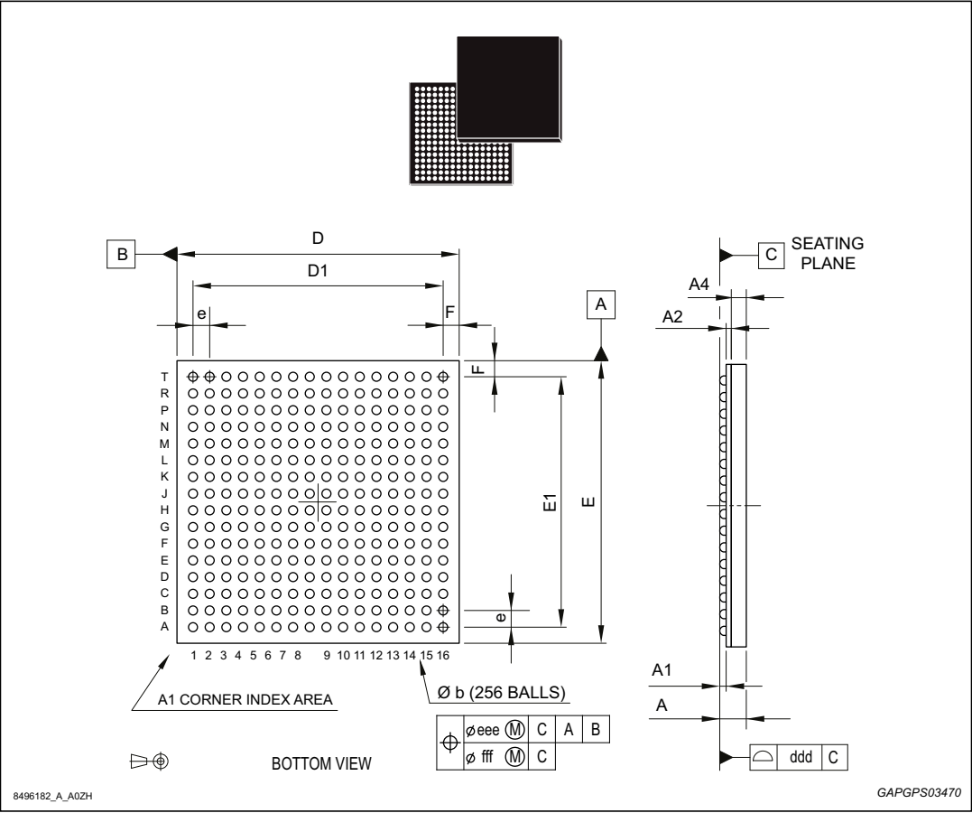
Figure 4. TFBGA256 (11x11x1.2 mm) package outline
