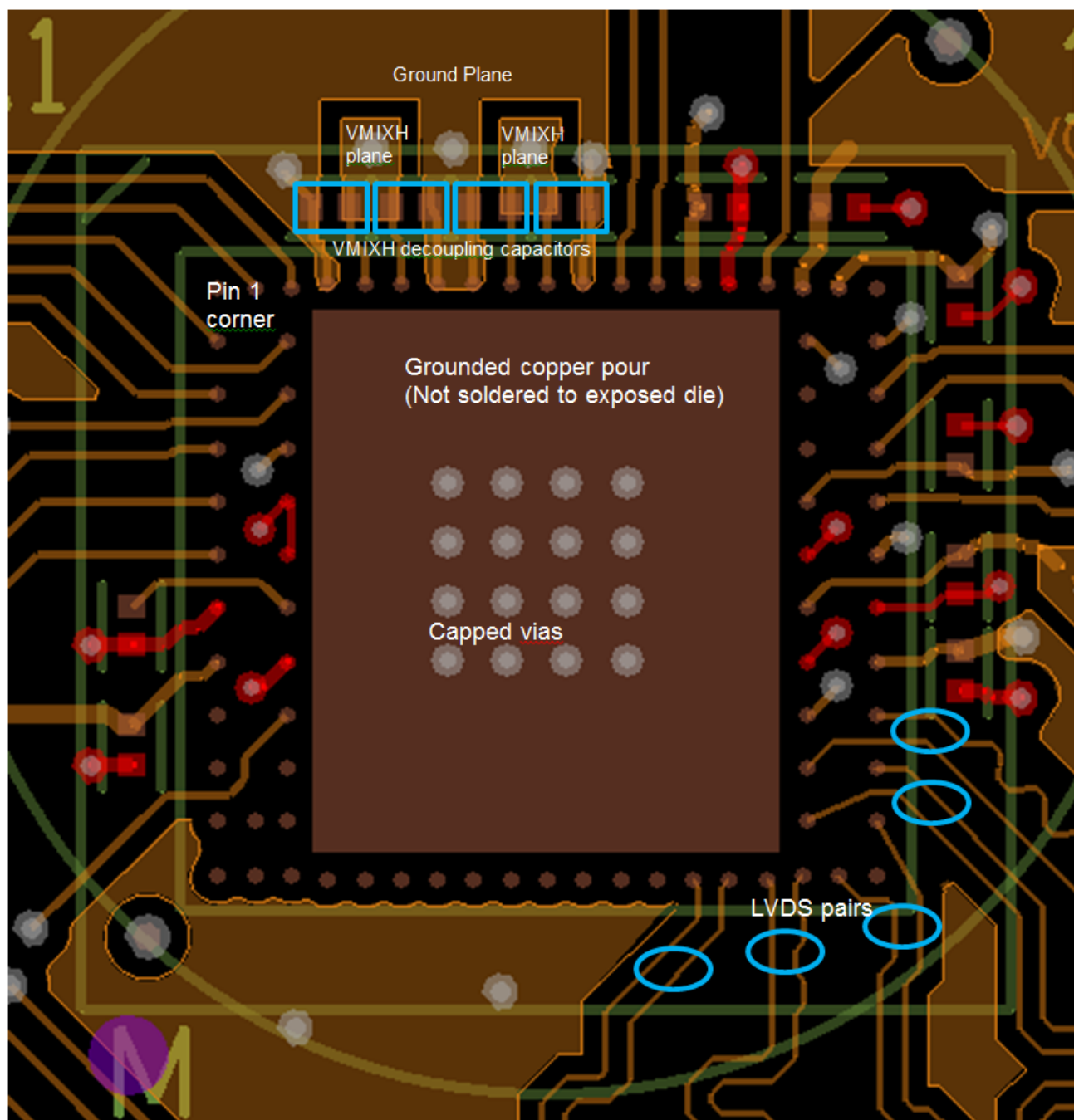
Figure 19. Example Layout
