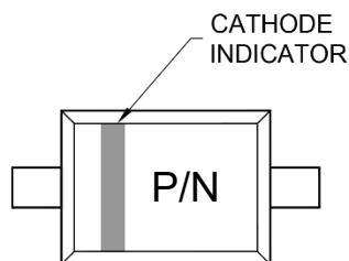
MARKING DIAGRAM
