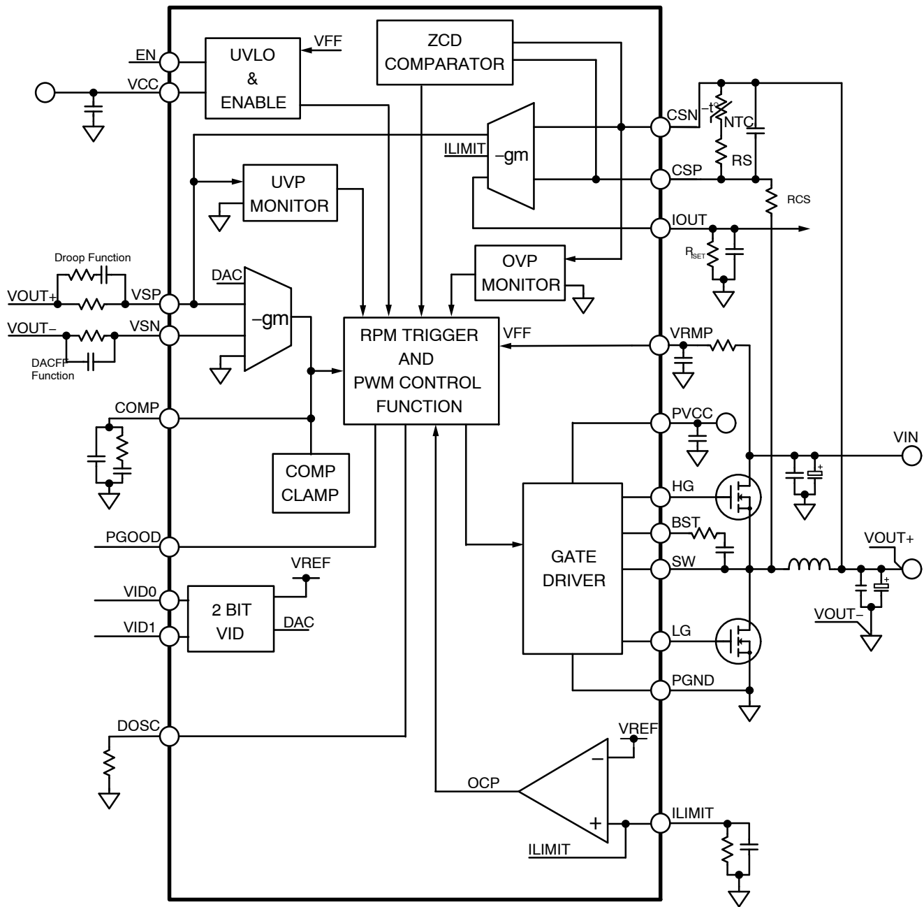
Figure 1. Block Diagram
