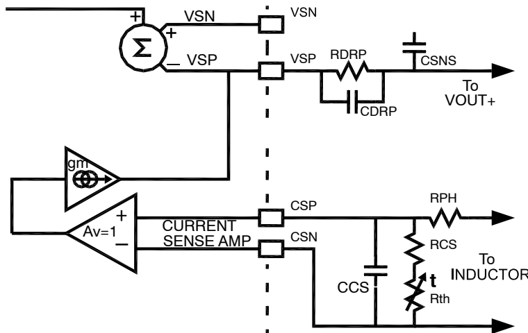
Figure 6. Droop Programming
