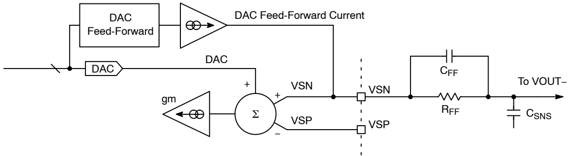
Figure 8. DAC Feed-Forward
