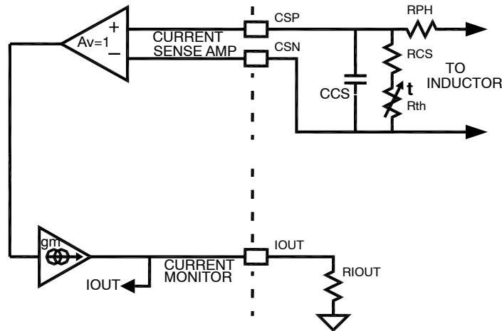
Figure 7. V_{IOUT} Programming
