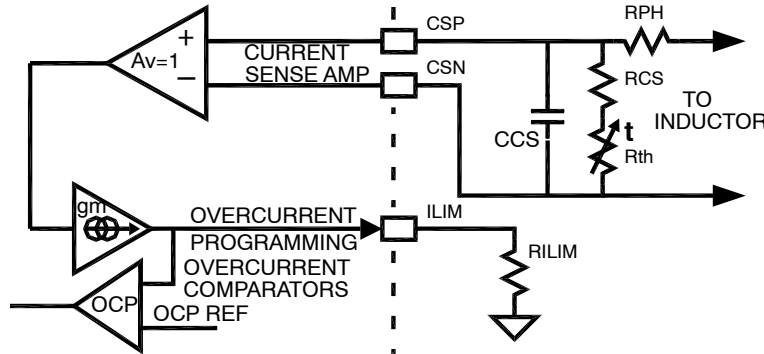
Figure 9. ILIM Programming
