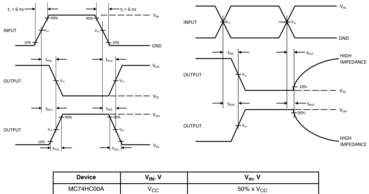
Figure 4. Switching Waveforms
