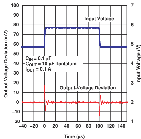
Figure 6-8. TLV1117-33 Line Transient Response
