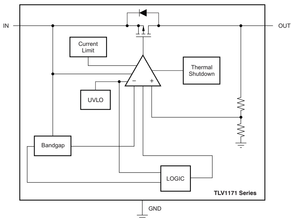
Figure 1. Block Diagram
