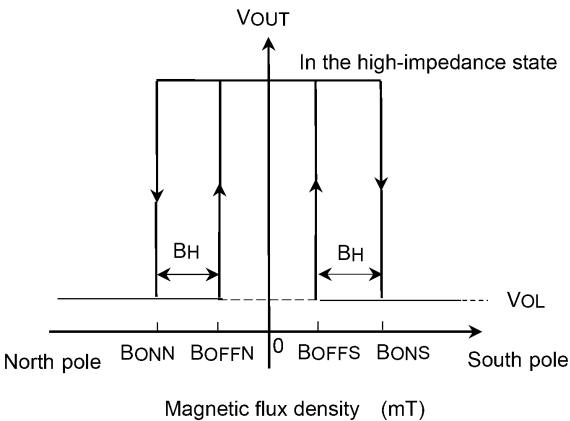
Fig. 8.2.2 Operating Characteristics
