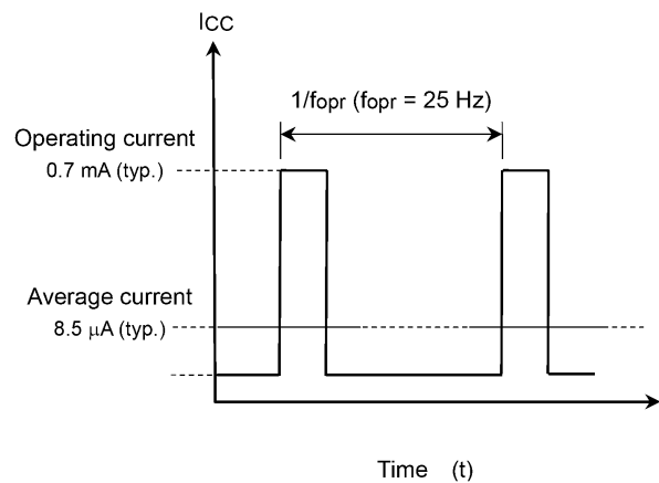
Fig. 8.1.1 I_{CC} Characteristics During Intermittent Operation
