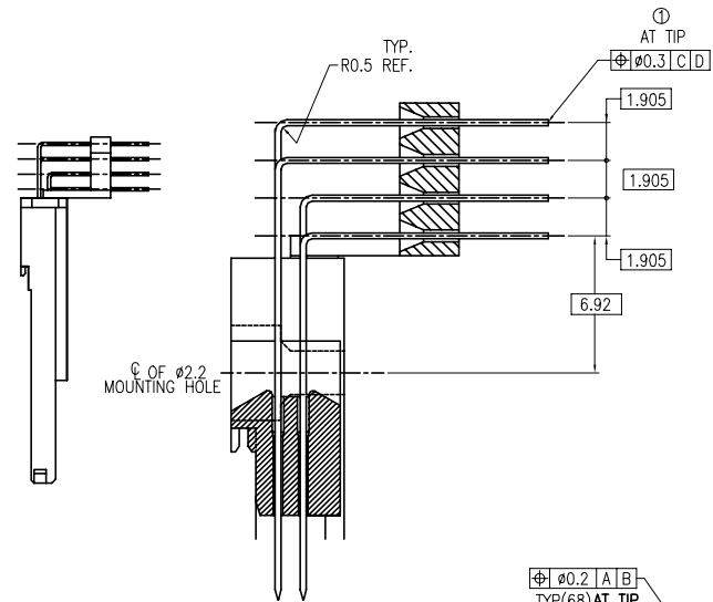
SECTION "Z-Z" (5/1)
