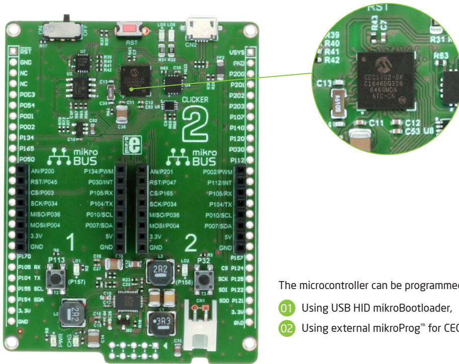
Figure 3-1: CEC1702 microcontroller
