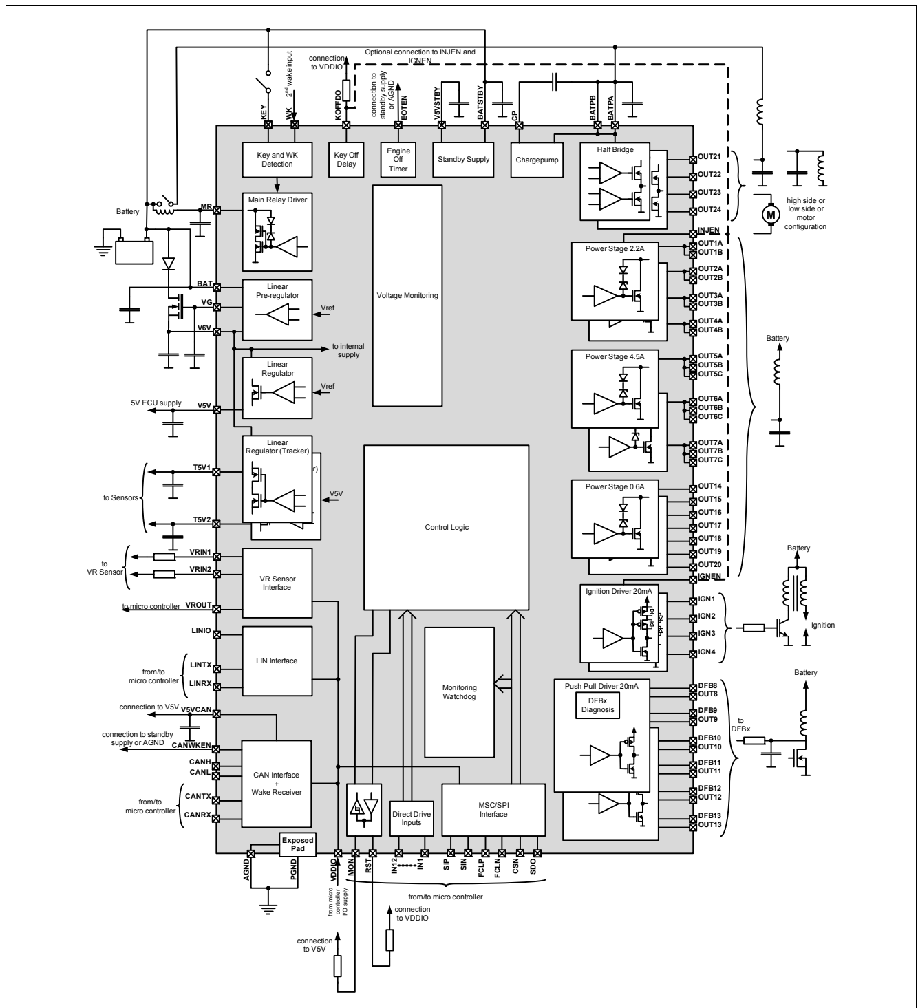
Figure 68 Application Diagram
