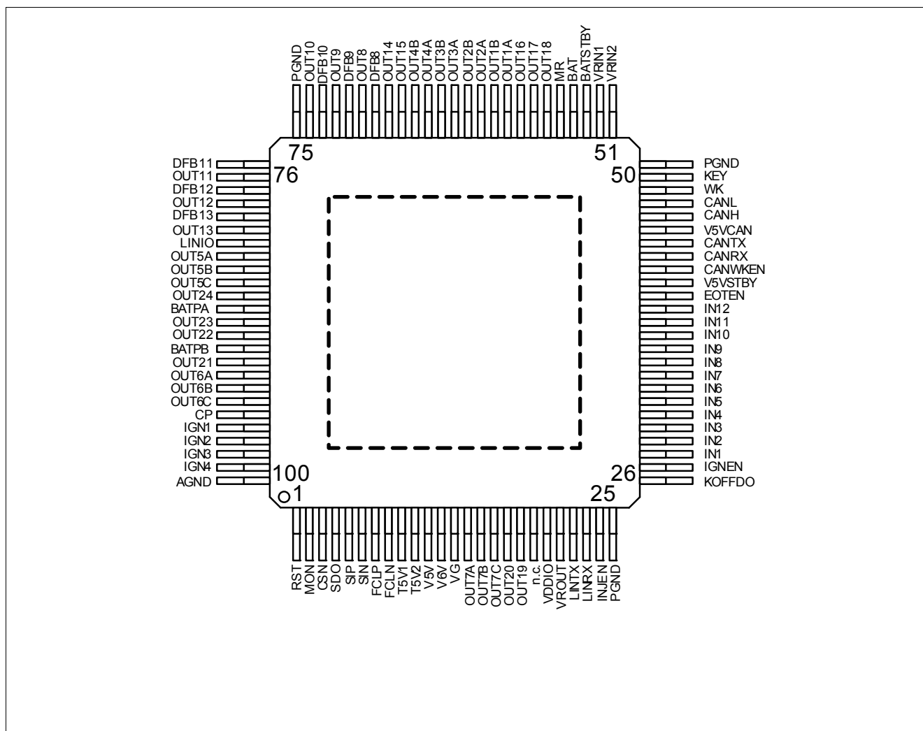
Figure 2 Pin Configuration
