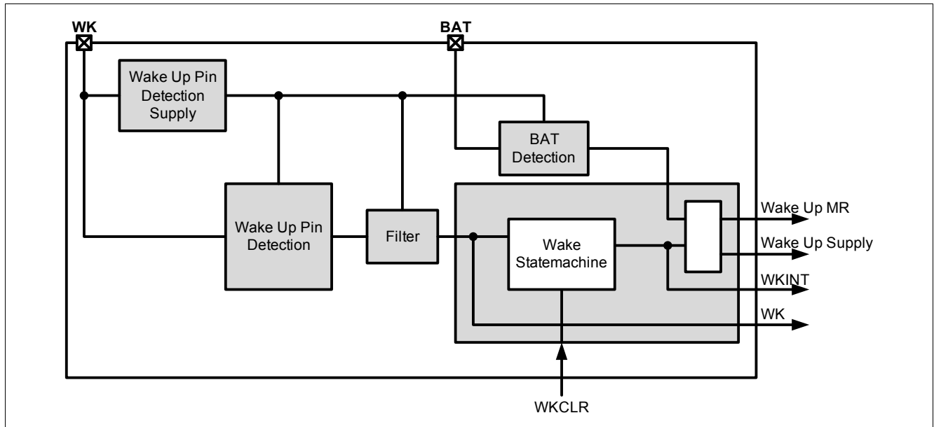
Figure 18 Block Diagram of the Wake Up Detection
