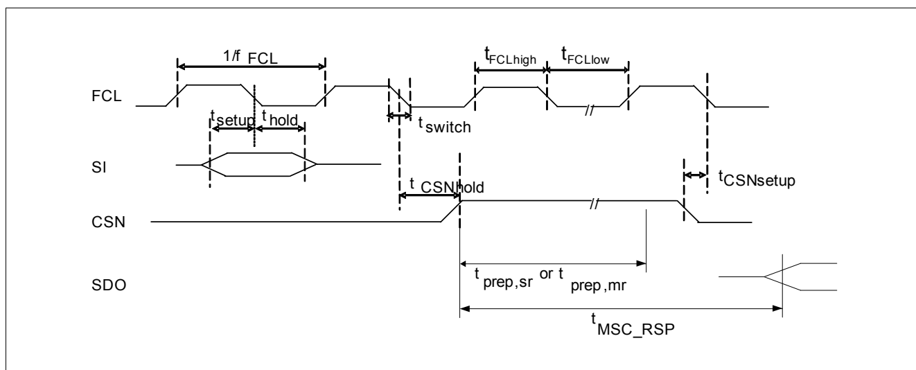
Figure 63 MSC timing
