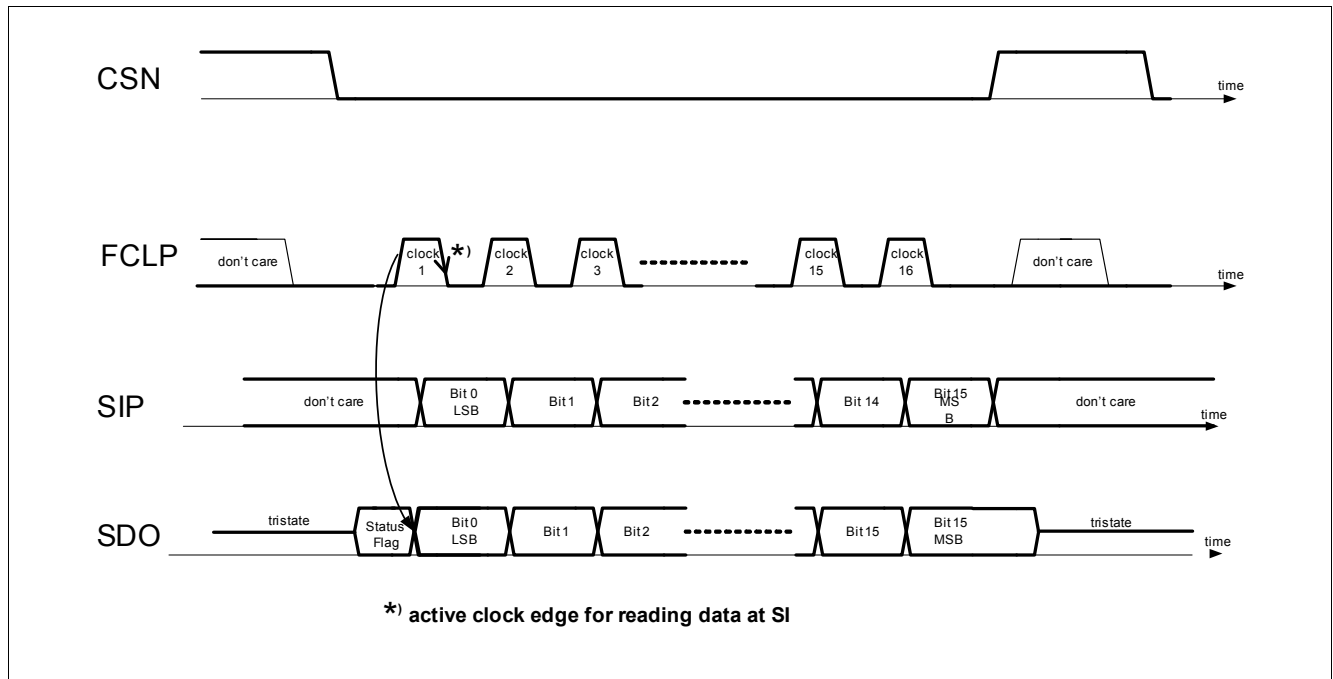
Figure 67 SPI Protocol
